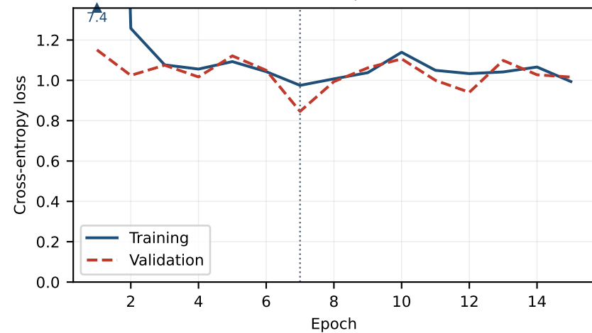
baseline (25,168,388 params)
