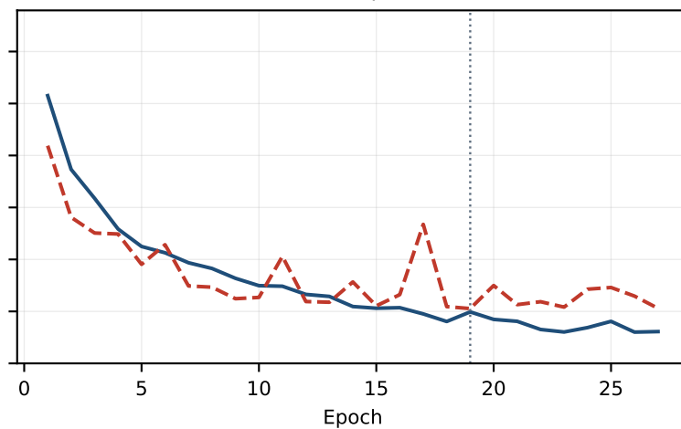
improved (1,290,404 params)
