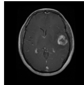
TRAIN Tr-gl_103.jpg (512, 512)
