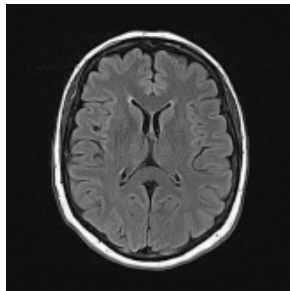
TRAIN Tr-no_803.jpg (442, 442)
