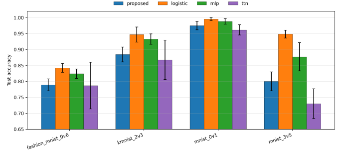
Fig. 4. Test accuracy of all arms on the four tasks (mean \pm standard deviation over five seeds).
