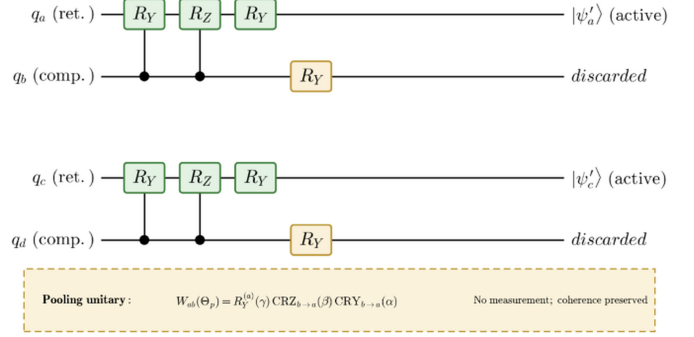
Fig. 3. Coherent unitary pooling mechanism. For each disjoint pair (a, b) \in P , qubit a is retained and b is compressed. The unitary W_{ab} transfers information from q_b into q_a via CRY and CRZ gates controlled on q_b and targeting q_a , followed by a local R_Y on each wire, with no mid-circuit measurement. The compressed qubit is excluded from all later operations; any unpaired wire is also retired by the executed schedule, while the global state remains pure before the active-register reduction.
