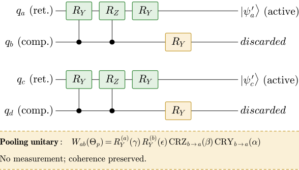
Fig. 3. Coherent unitary pooling mechanism. For each disjoint pair (a, b) \in P , qubit a is retained and b is compressed. The unitary W_{ab} transfers information from q_b into q_a via CRY and CRZ gates controlled on q_b and targeting q_a , followed by a local R_Y on each wire, with no mid-circuit measurement. The compressed qubit is excluded from all later operations; any unpaired wire is also retired by the executed schedule, while the global state remains pure before the active-register reduction.
