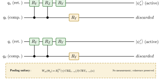
Fig. 3. Coherent unitary pooling mechanism. For each disjoint pair (a, b) \in P , qubit a is retained and b is compressed. The unitary W_{ab} transfers information from q_b into q_a via CRY and CRZ gates controlled on q_b and targeting q_a , followed by a local R_Y on each wire, with no mid-circuit measurement. The compressed qubit is excluded from all later operations; any unpaired wire is also retired by the executed schedule, while the global state remains pure before the active-register reduction.
