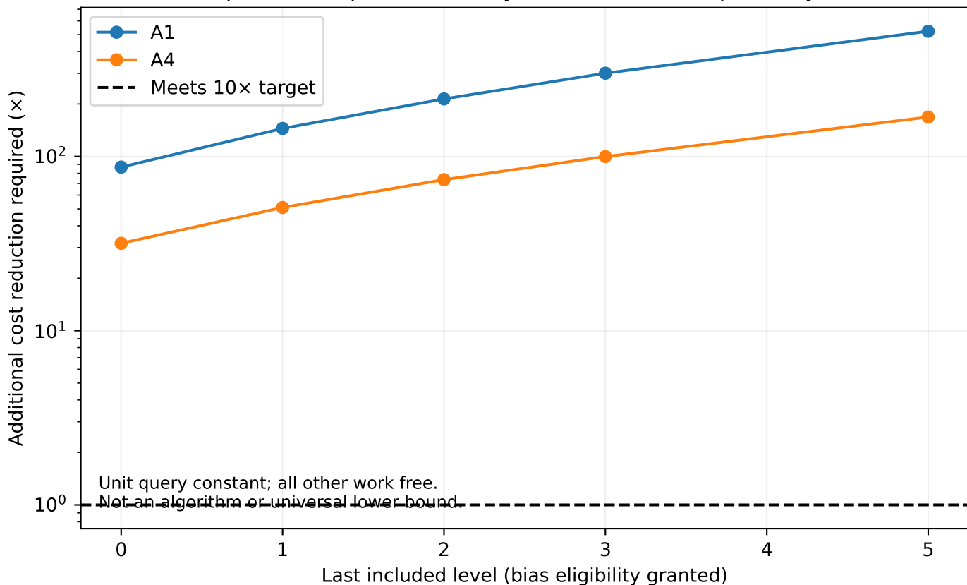
Optimistic square-root-only screen at 100 ns per T layer
