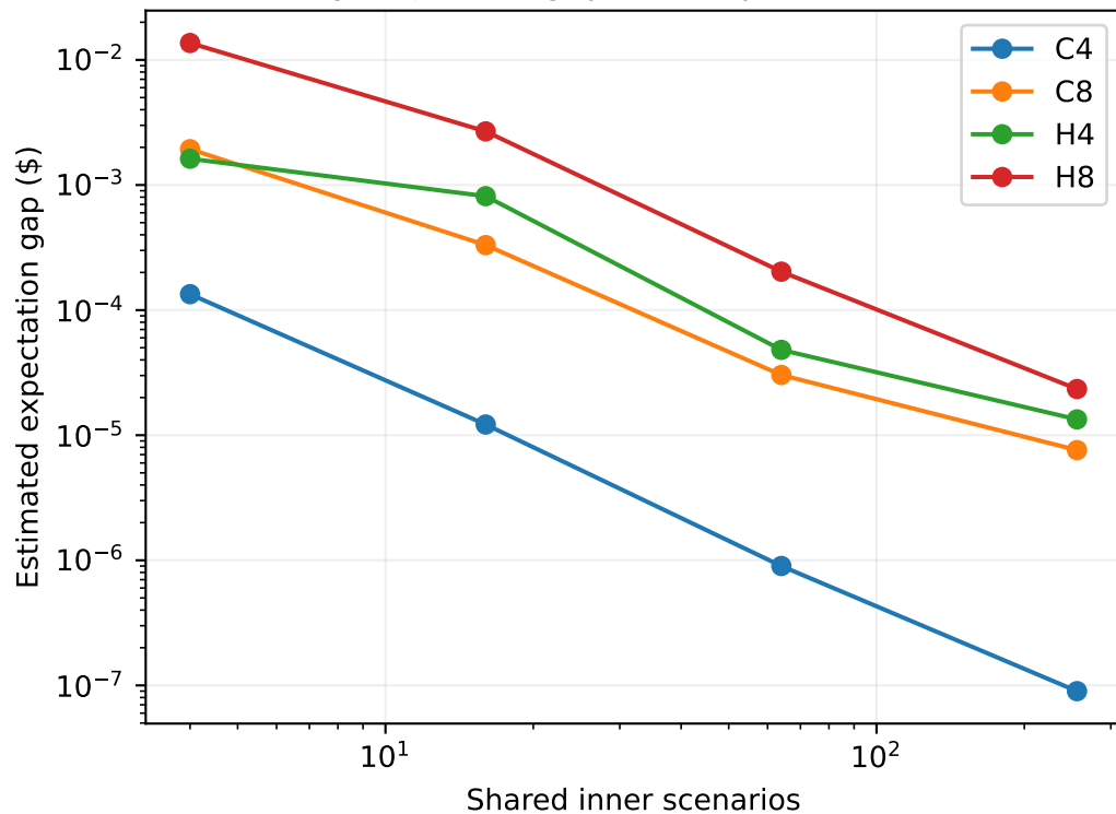
Policy-to-Jensen gap at compound strike $6
