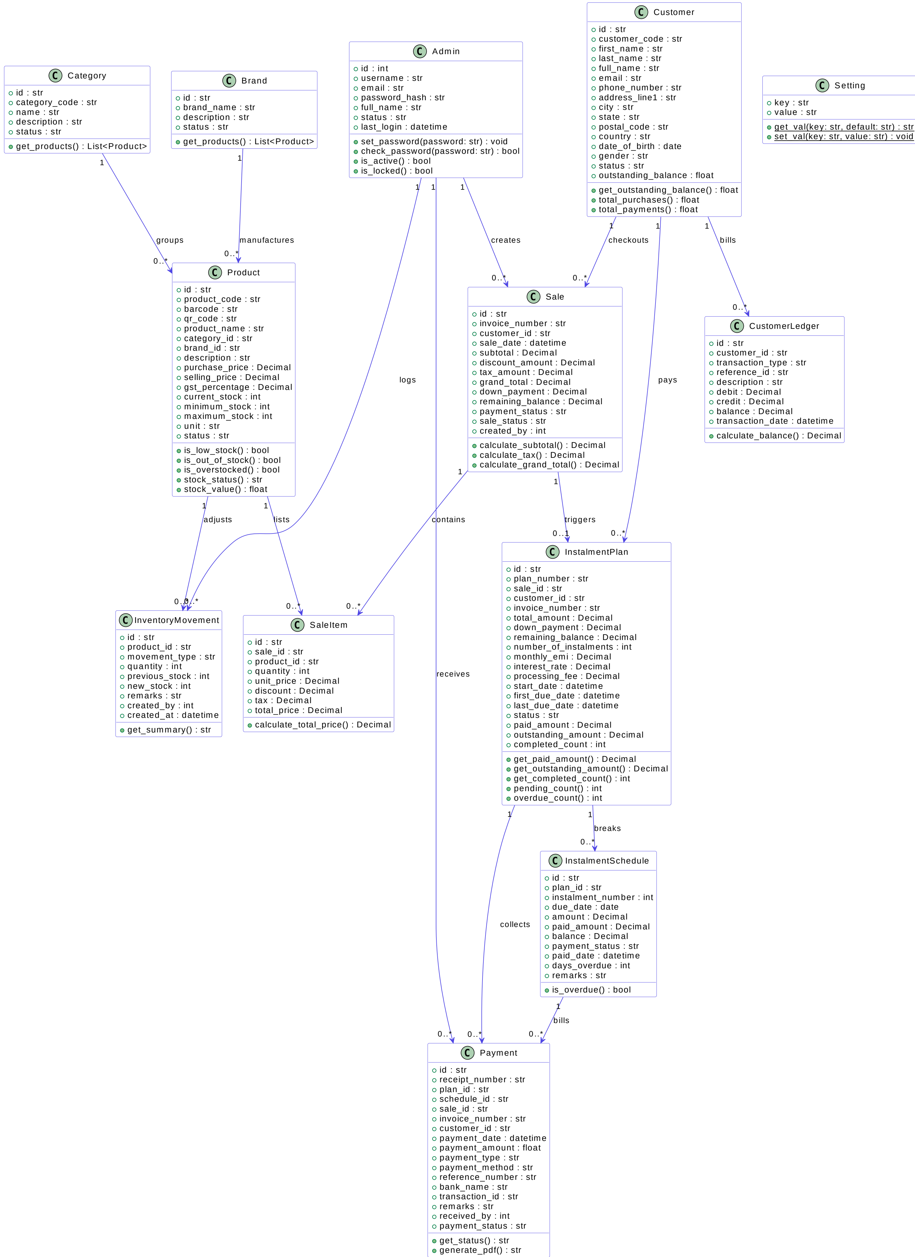
PayEase - UML Class Diagram
