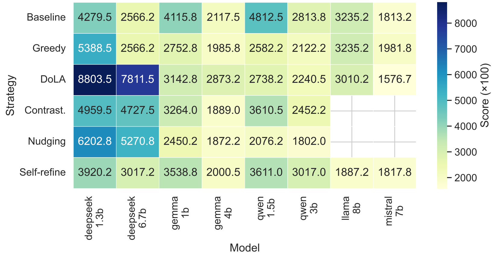
PHR (%) without stdlib: Strategy × Model
