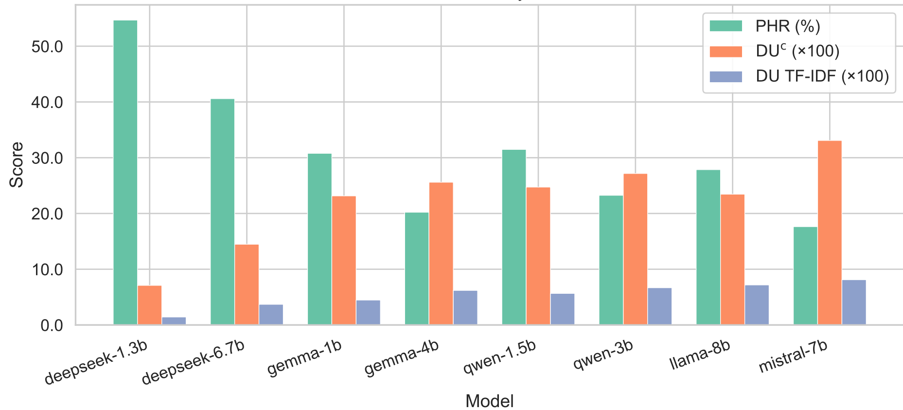
PHR and DU by Model
