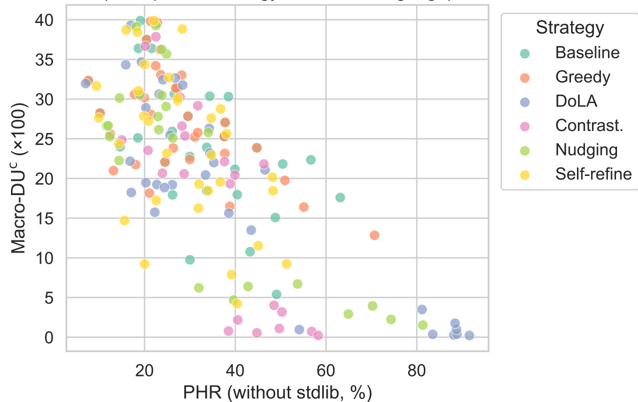
Safety–Utility Trade-off (each point = strategy × model × language)
