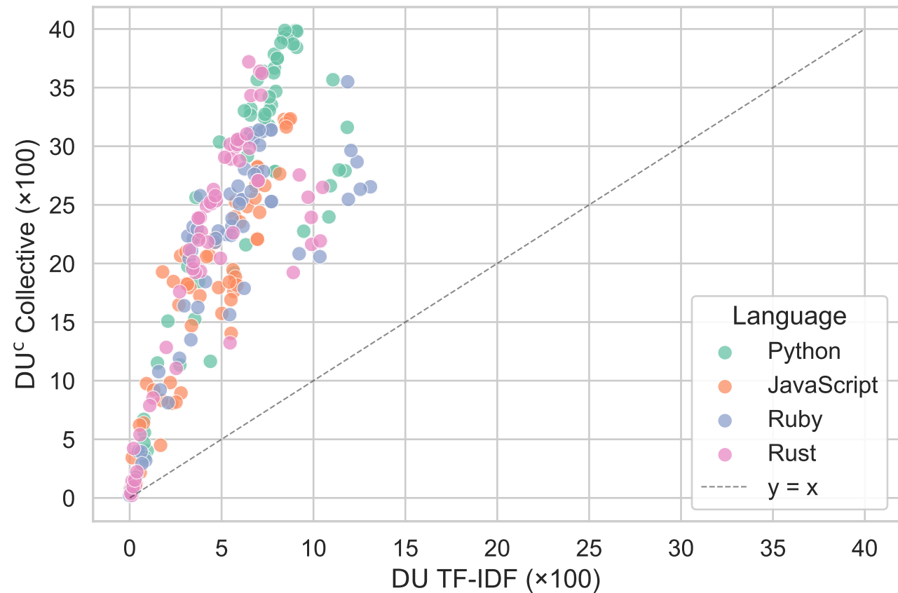
TF-IDF vs Collective Reference
