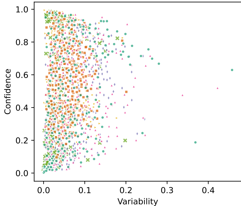
Stable Code-3B
