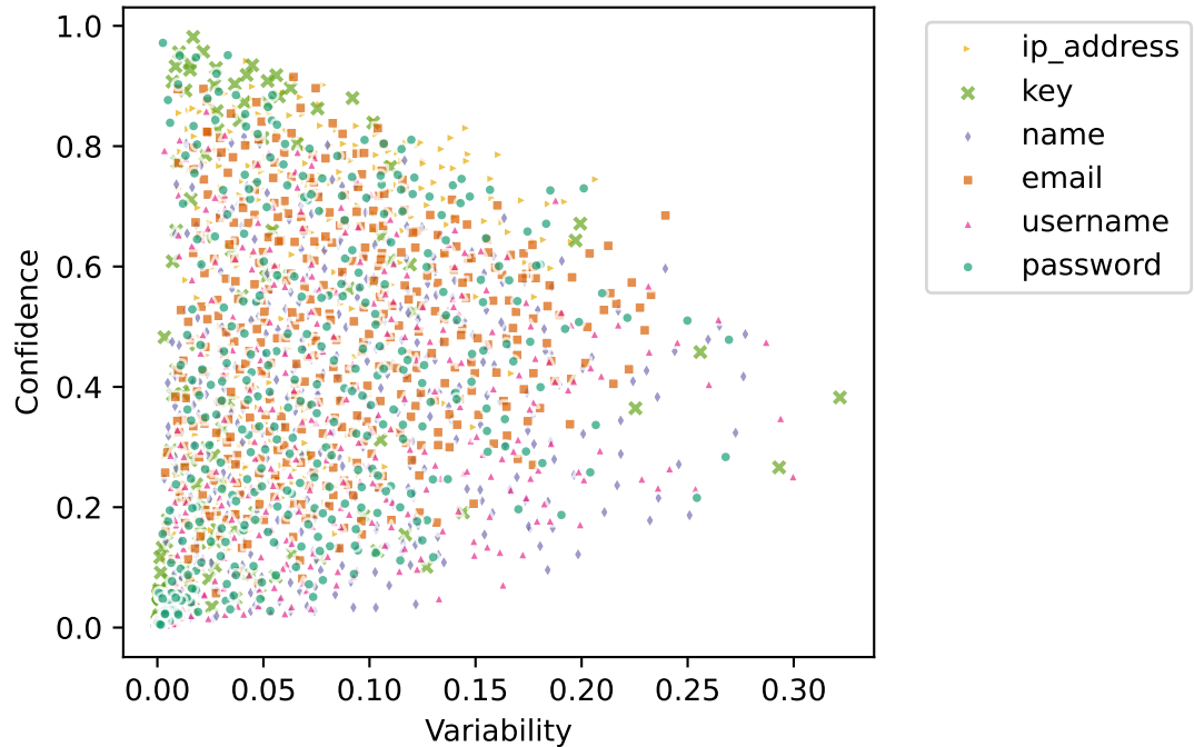
Qwen2.5 Coder-3B
