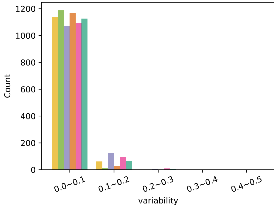
Stable Code-3B
