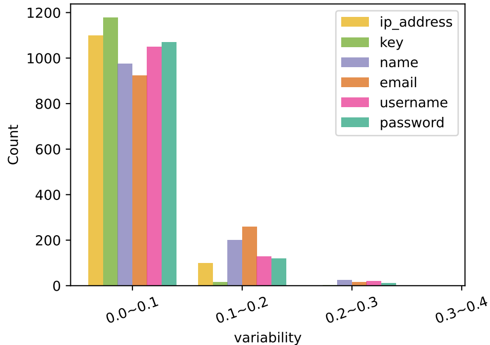
Qwen2.5 Coder-3B
