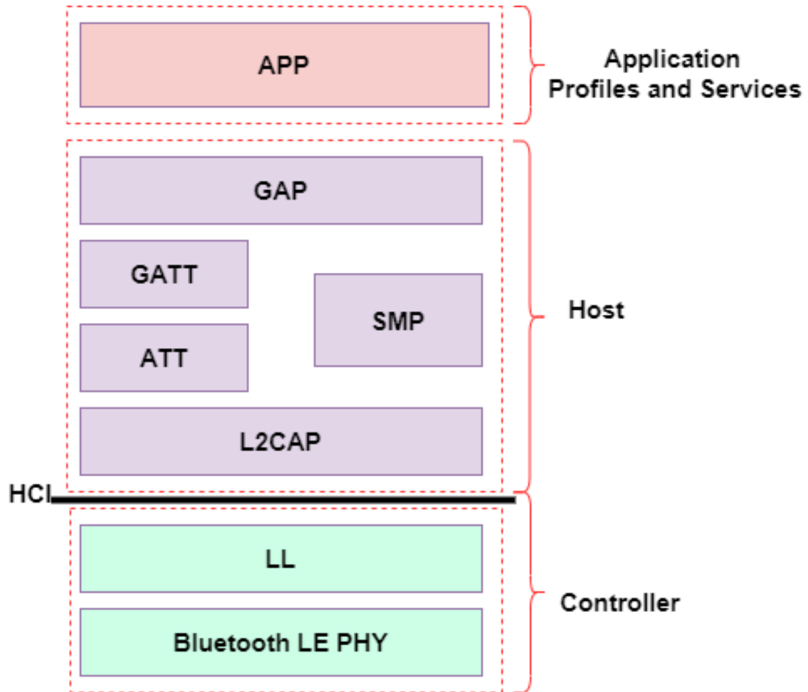
Figure 2: BLE protocol stack ( https://de.mathworks.com/help/bluetooth/gs/bluetooth-protocol-stack.html )
