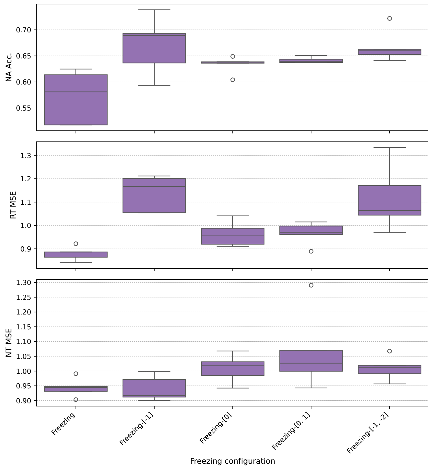
BPI20TravelPermitData - gptneo-1b3 (Freezing variants)
