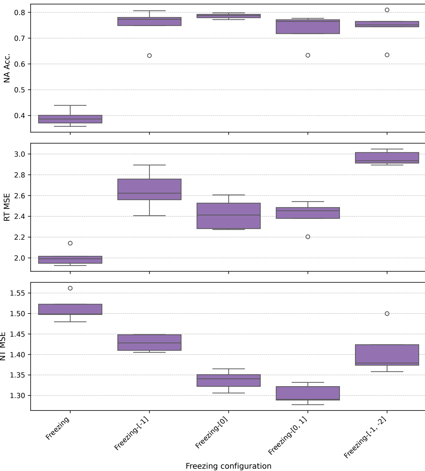
BPI12 - gemma-2-2b (Freezing variants)
