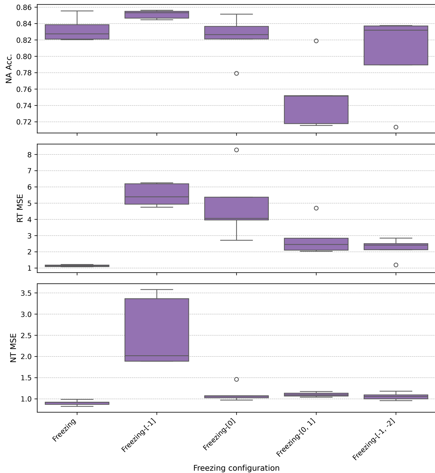
BPI17 - llama32-1b (Freezing variants)
