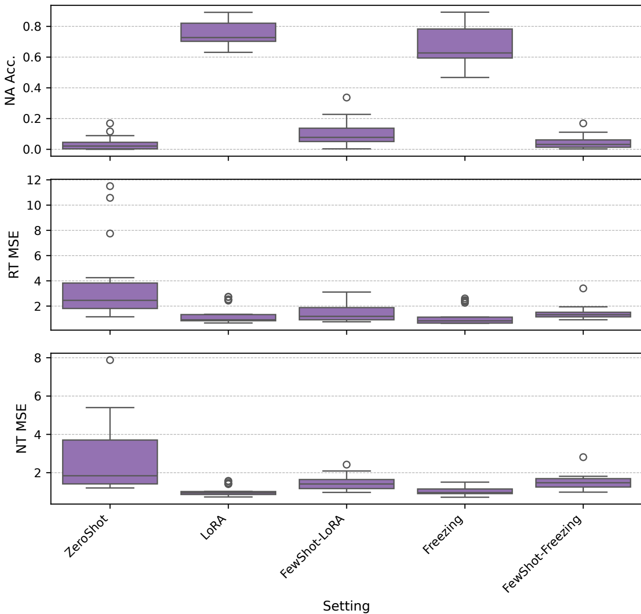
Backbone: gpt2
