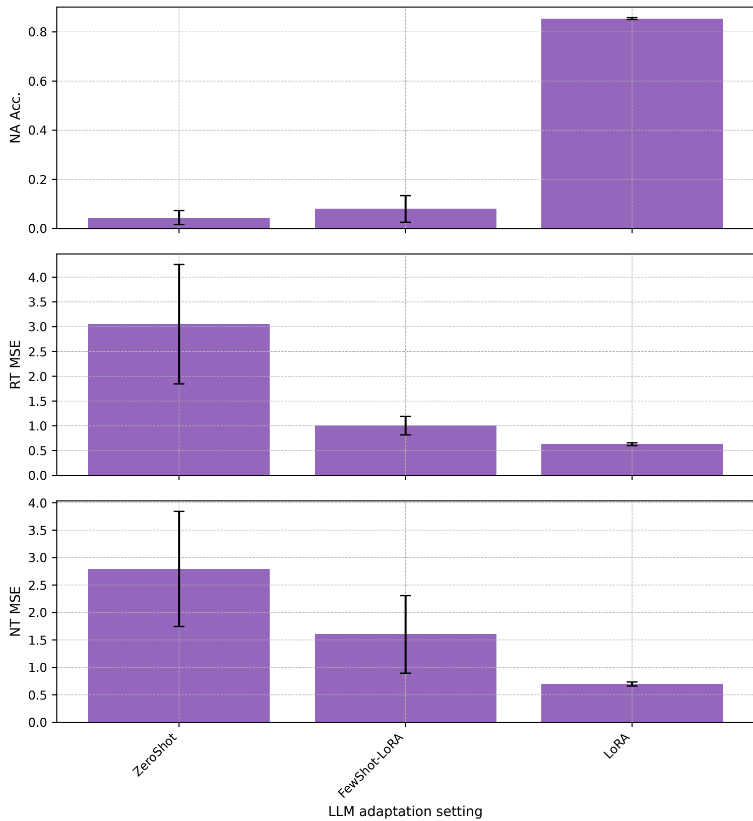
BPI17 - qwen25-05b
