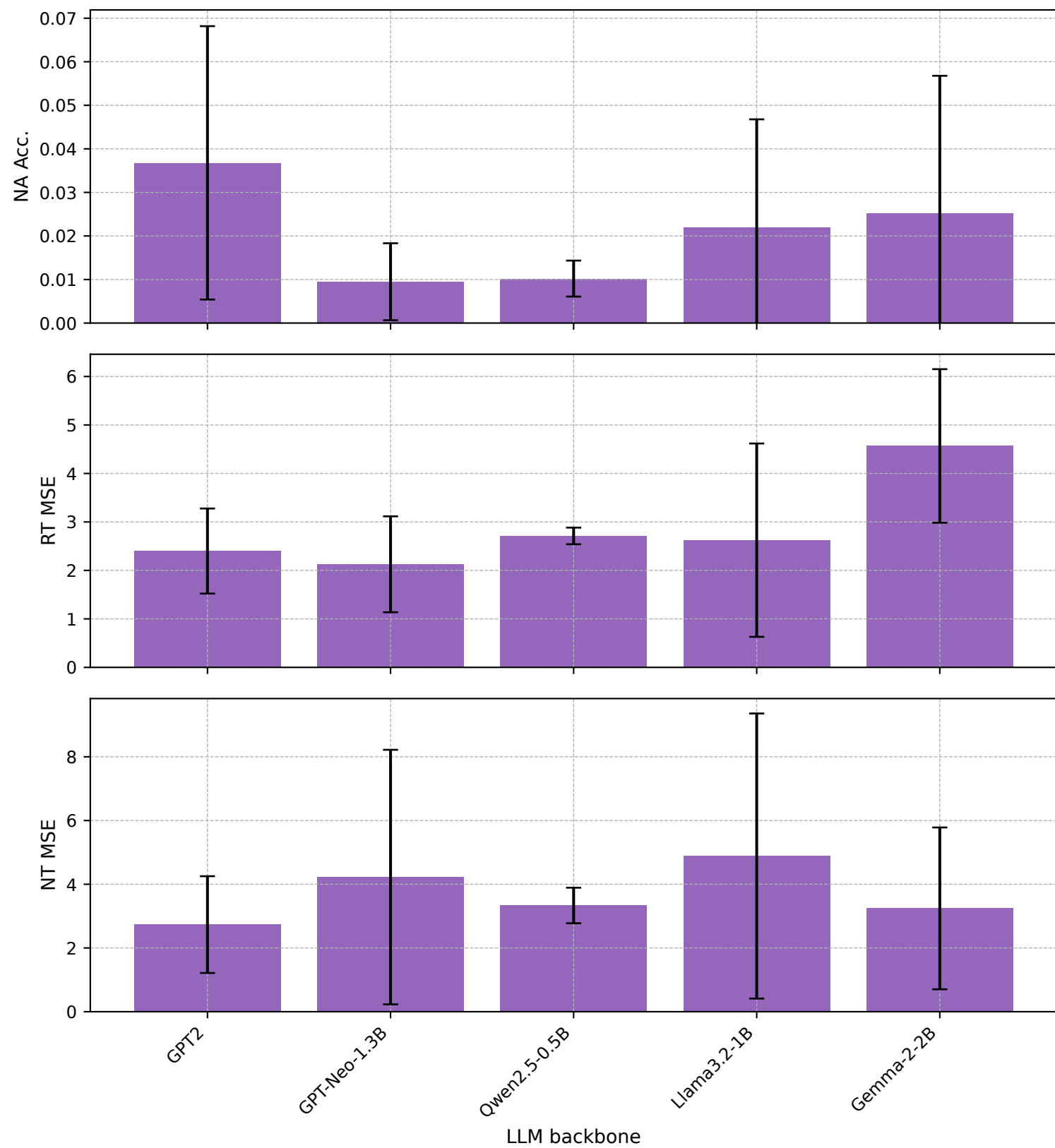
BPI20TravelPermitData - ZeroShot
