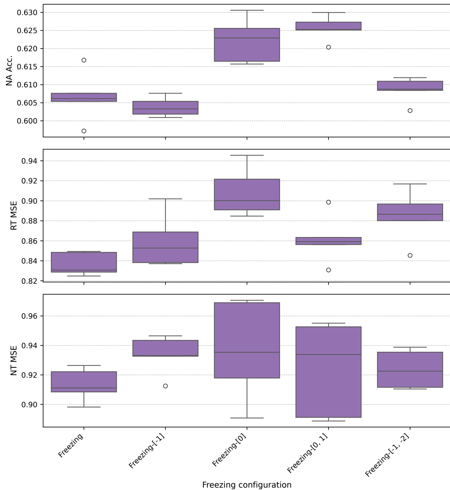
BPI20TravelPermitData - gpt2 (Freezing variants)
