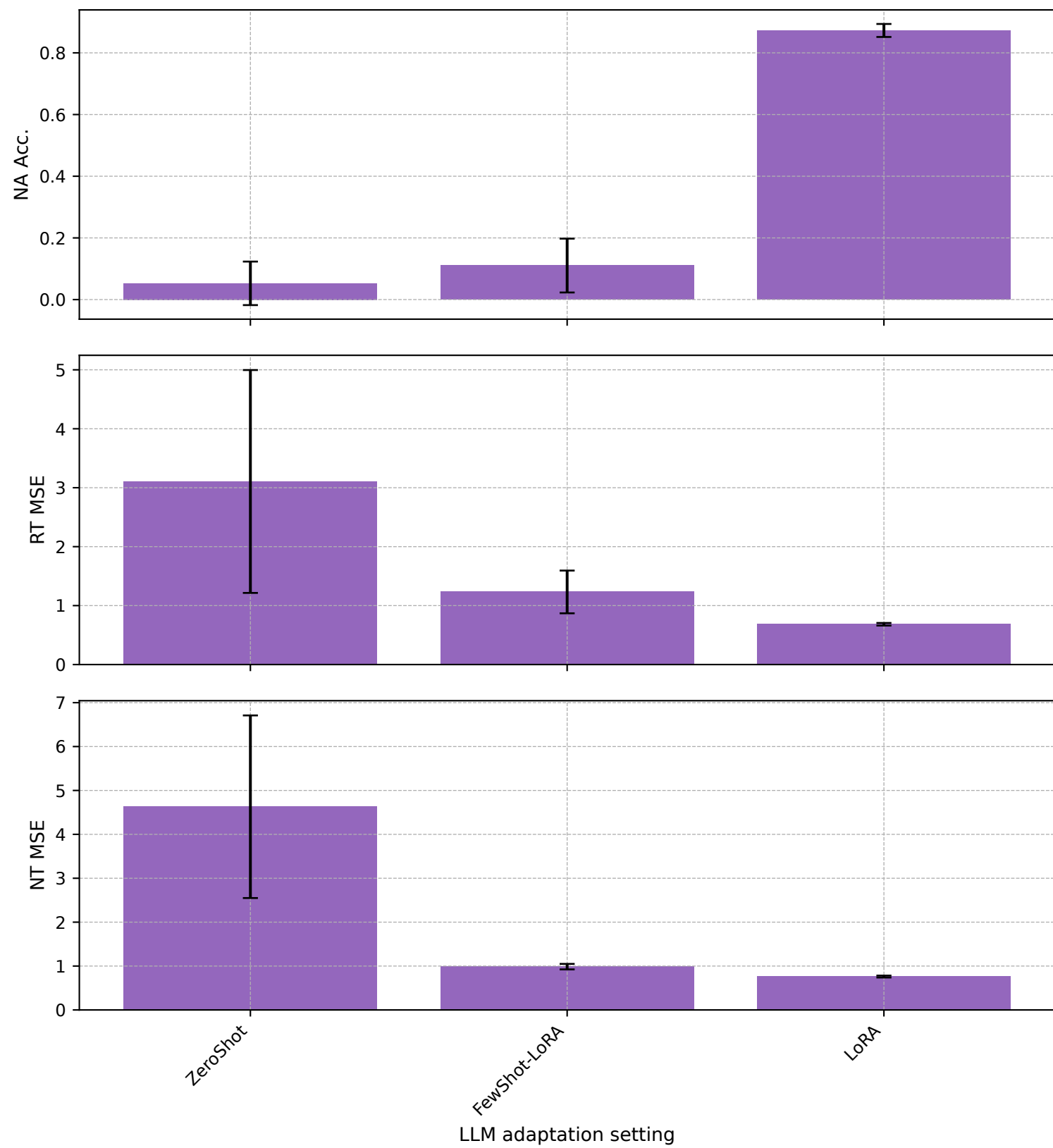
BPI20RequestForPayment - gptneo-1b3
