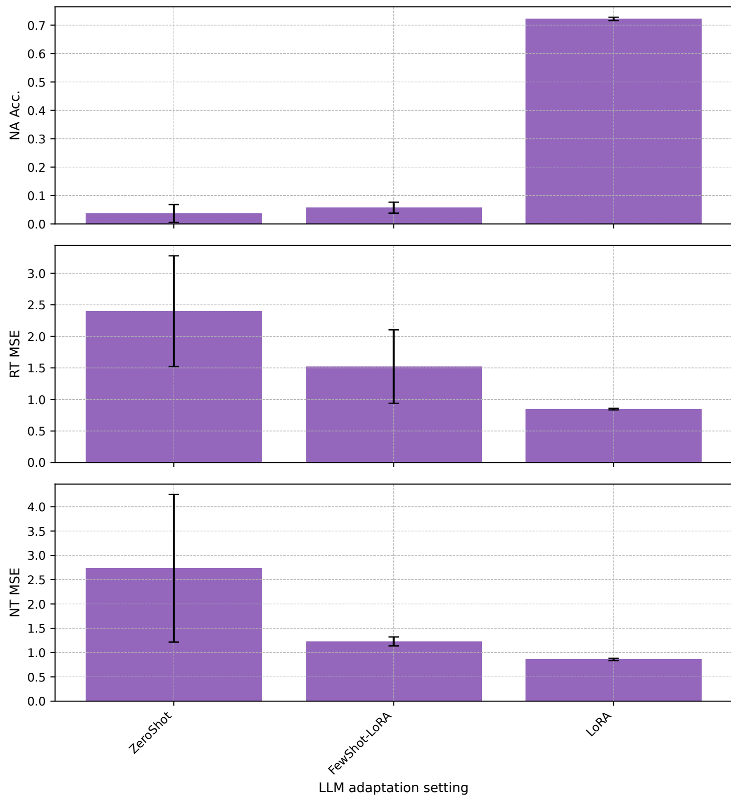
BPI20TravelPermitData - gpt2
