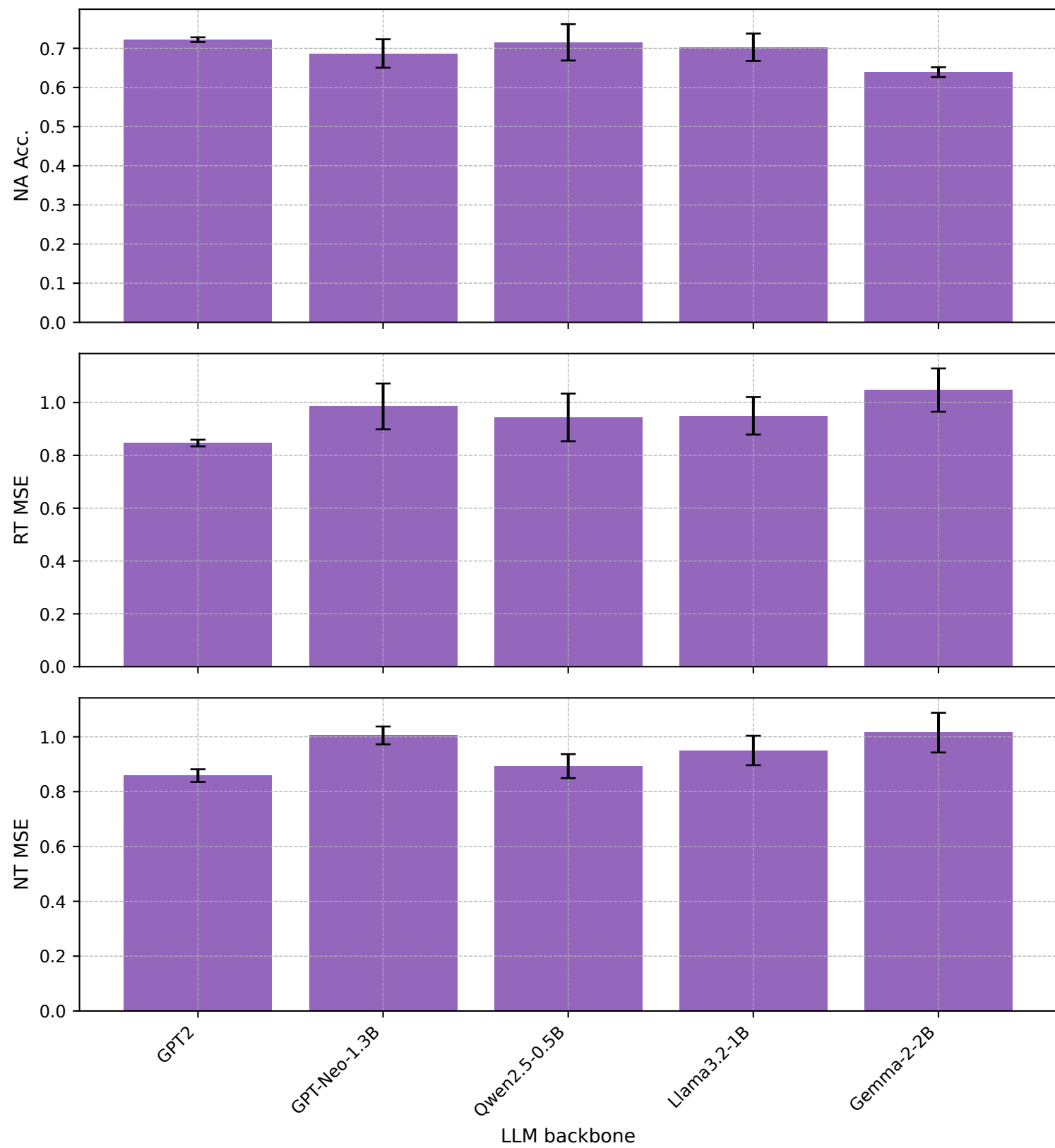
BPI20TravelPermitData - LoRA
