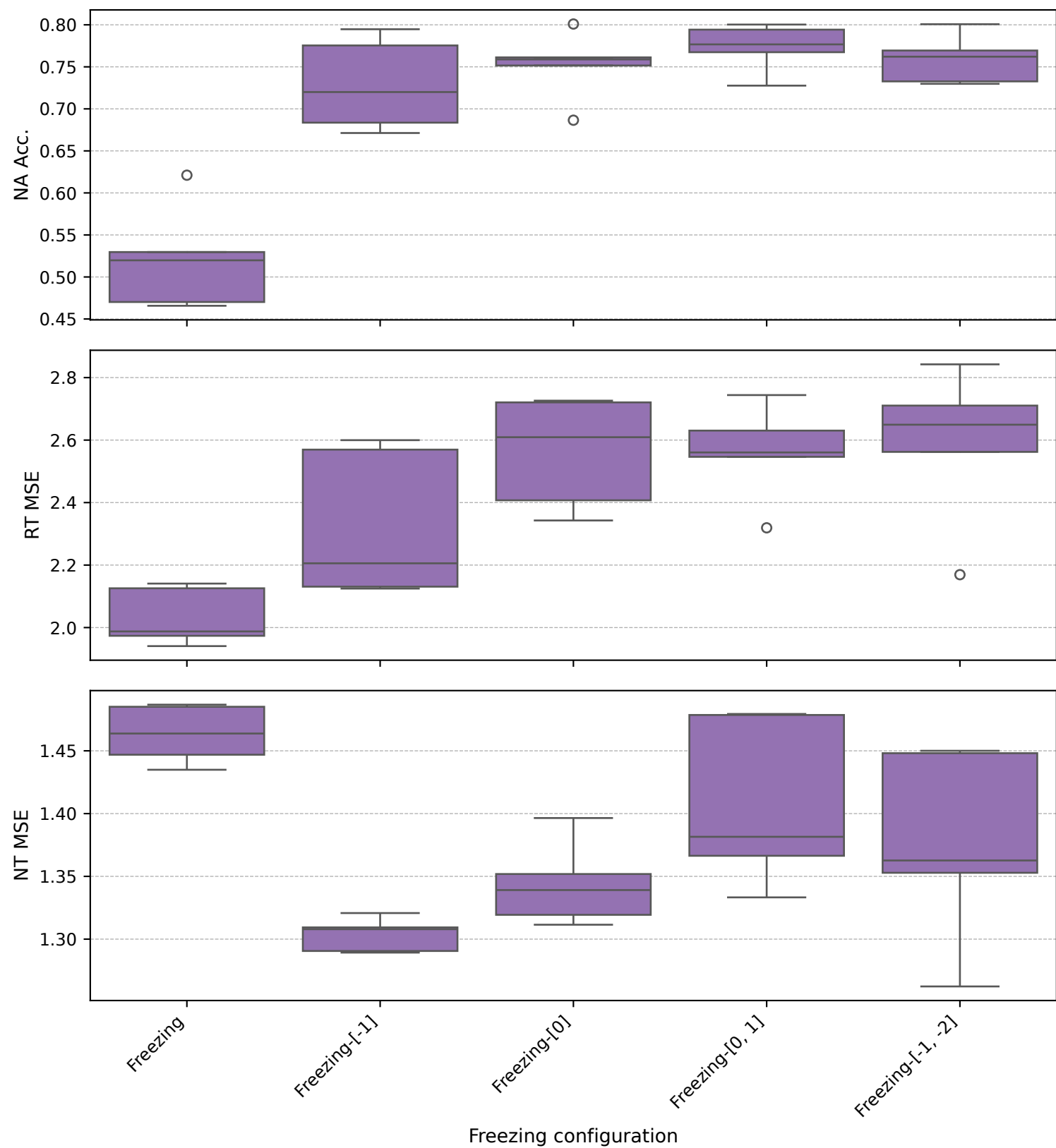
BPI12 - llama32-1b (Freezing variants)
