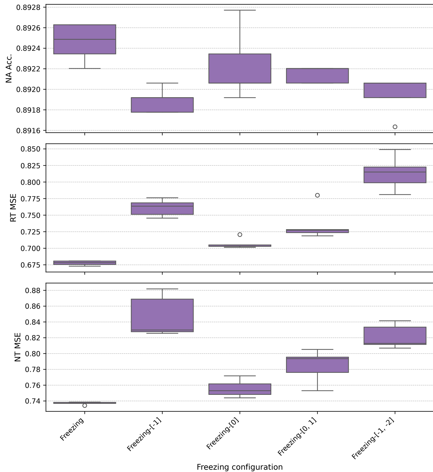
BPI20RequestForPayment - gemma-2-2b (Freezing variants)
