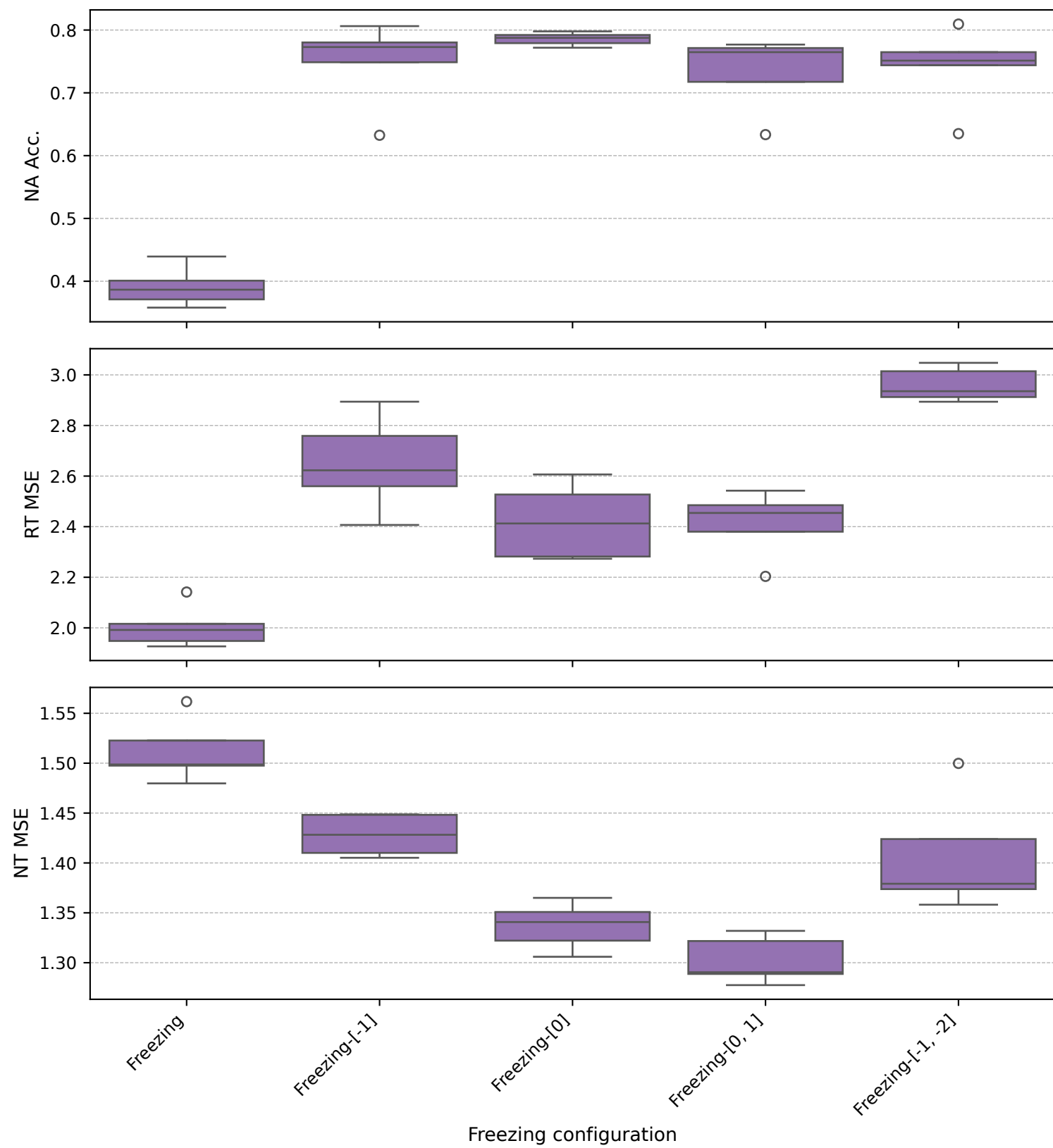
BPI12 - gemma-2-2b (Freezing variants)
