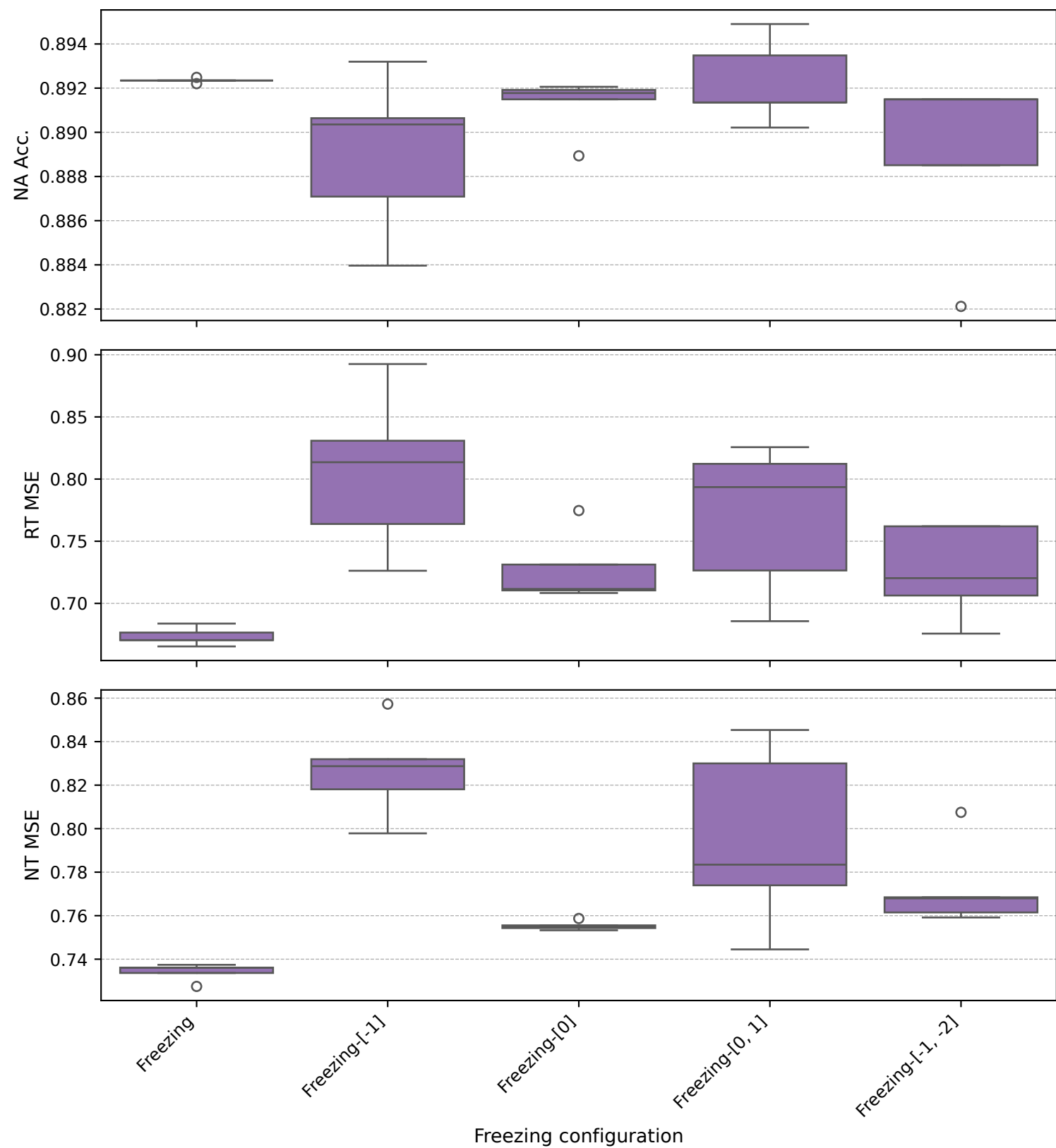
BPI20RequestForPayment - llama32-1b (Freezing variants)
