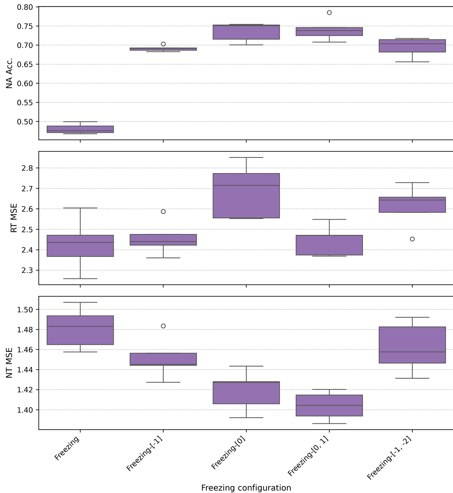
BPI12 - gpt2 (Freezing variants)
