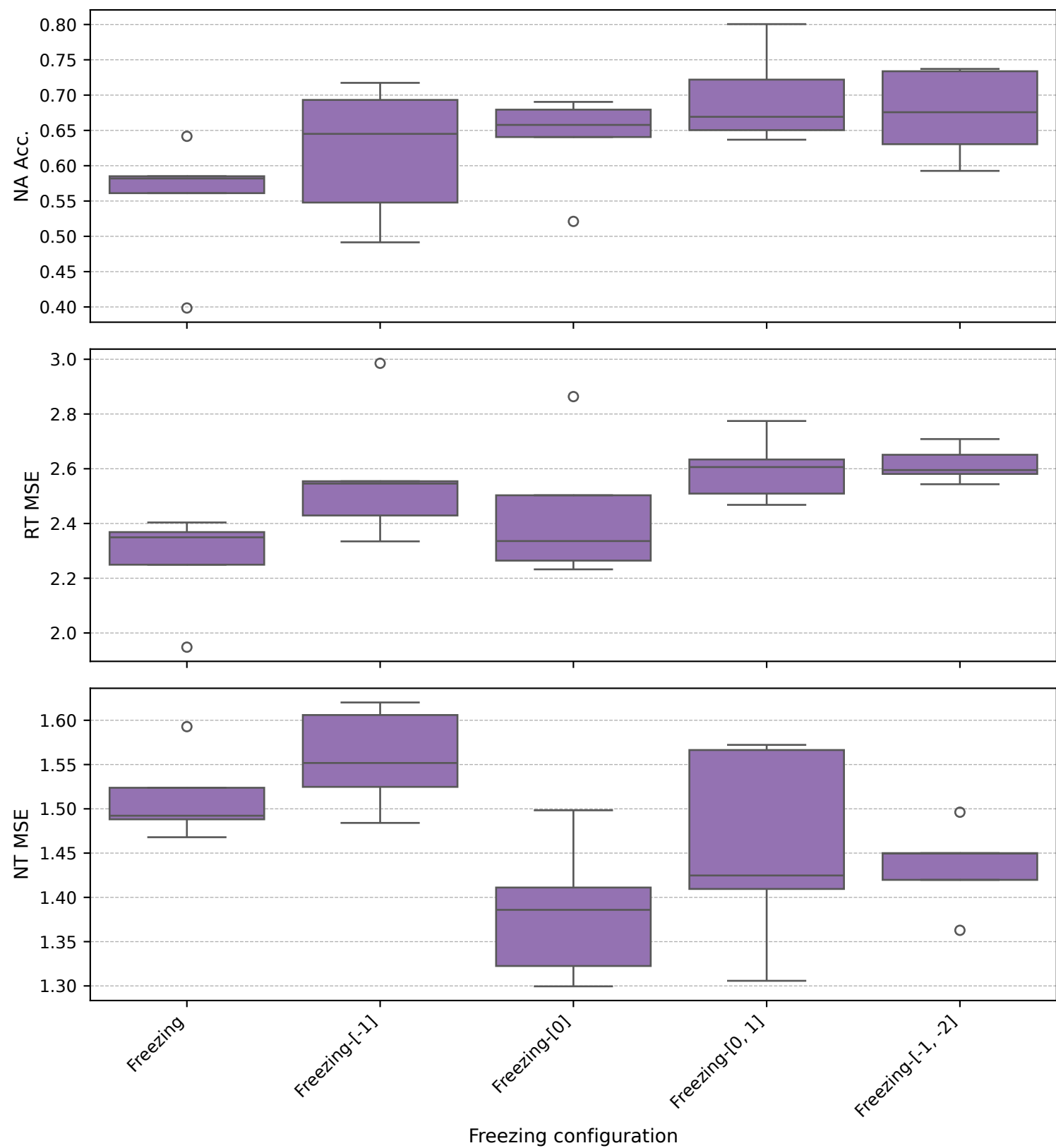
BPI12 - qwen25-05b (Freezing variants)
