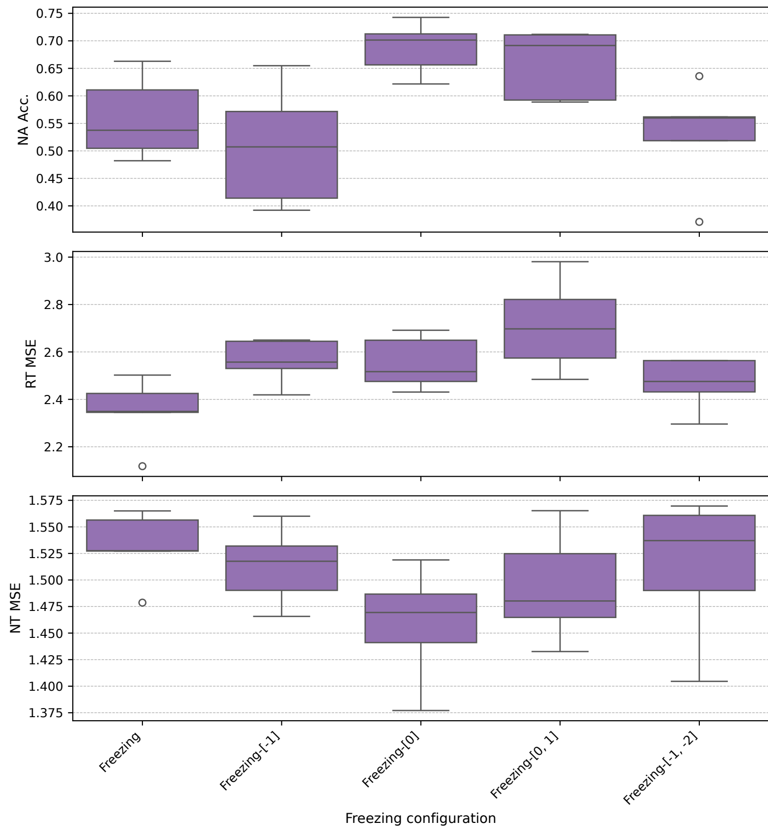
BPI12 - gptneo-1b3 (Freezing variants)
