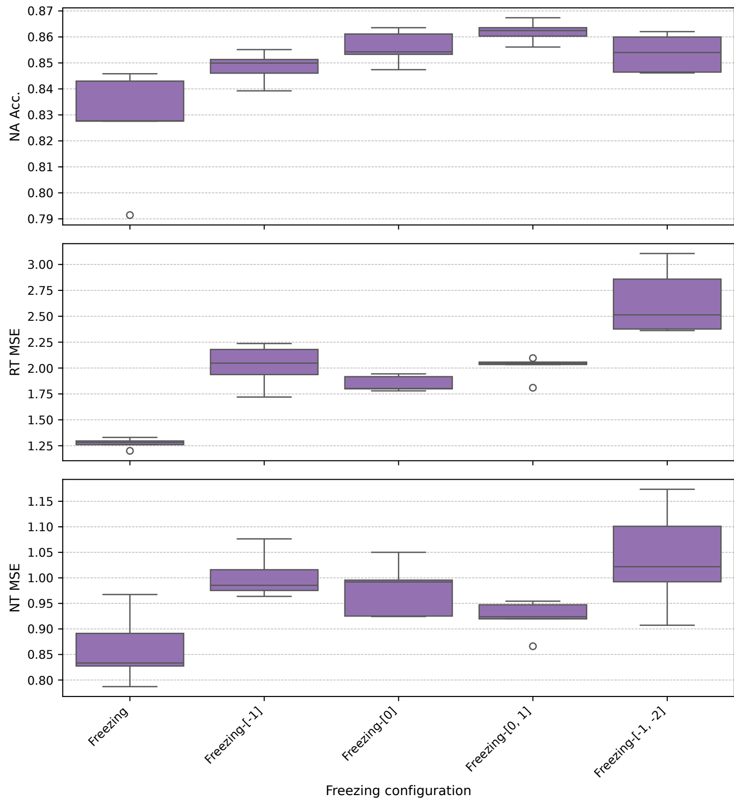
BPI17 - gemma-2-2b (Freezing variants)
