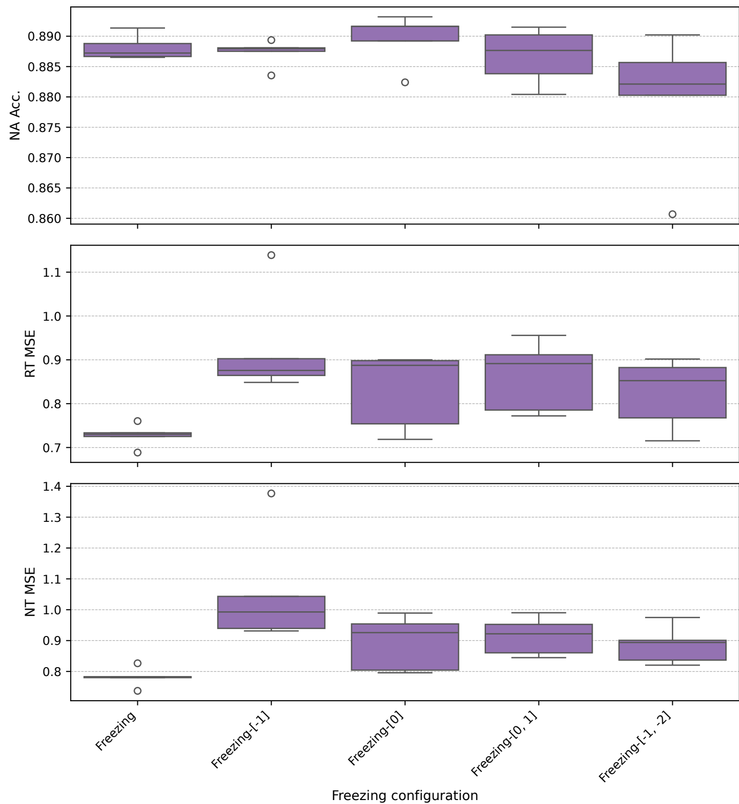
BPI20RequestForPayment - qwen25-05b (Freezing variants)
