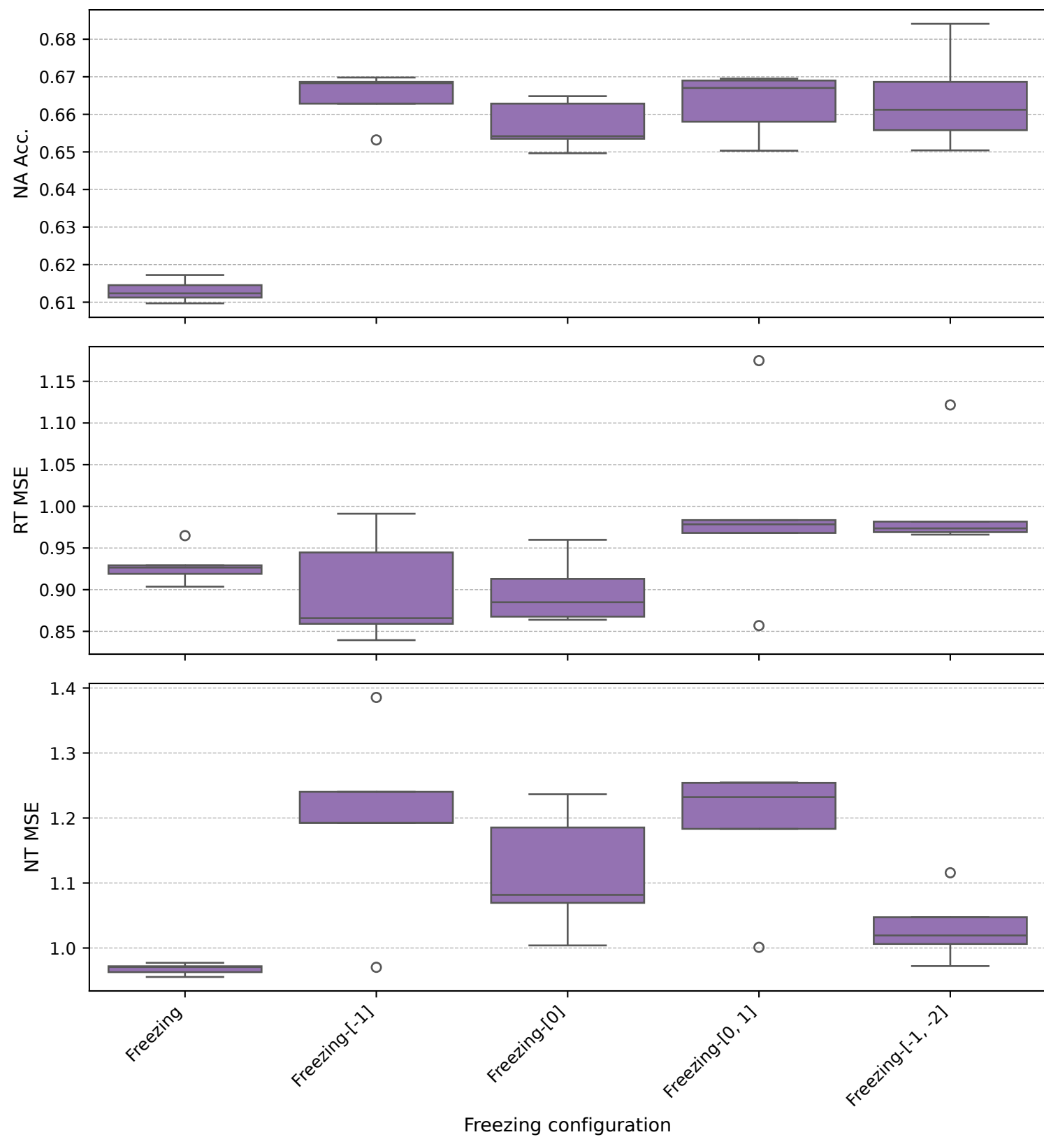
BPI20TravelPermitData - llama32-1b (Freezing variants)
