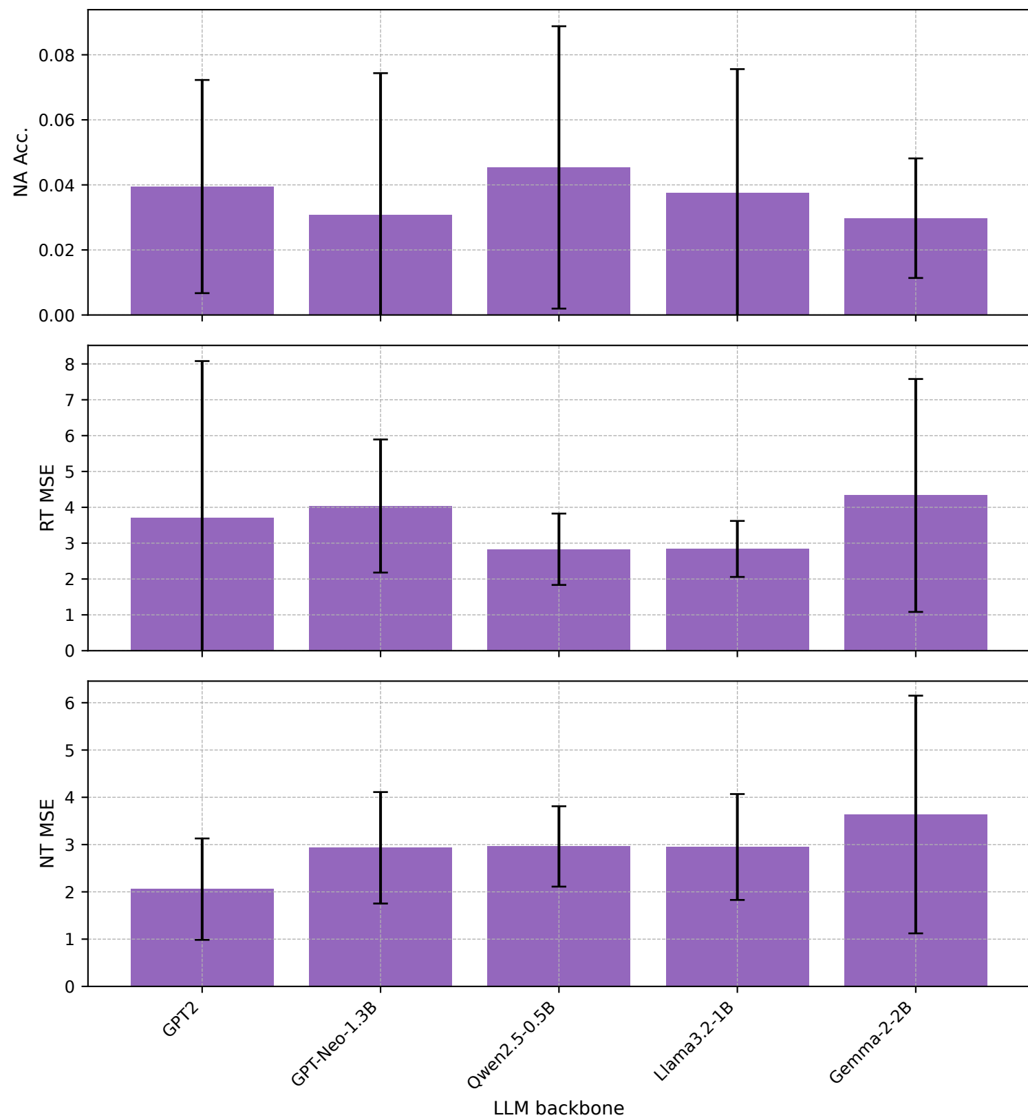
BPI12 - ZeroShot
