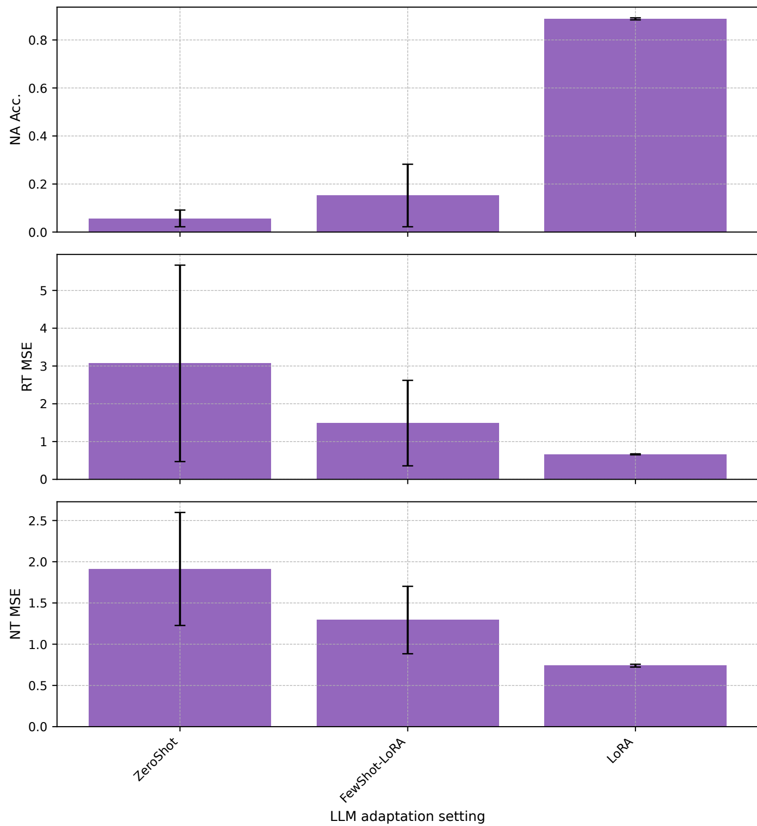
BPI20RequestForPayment - qwen25-05b
