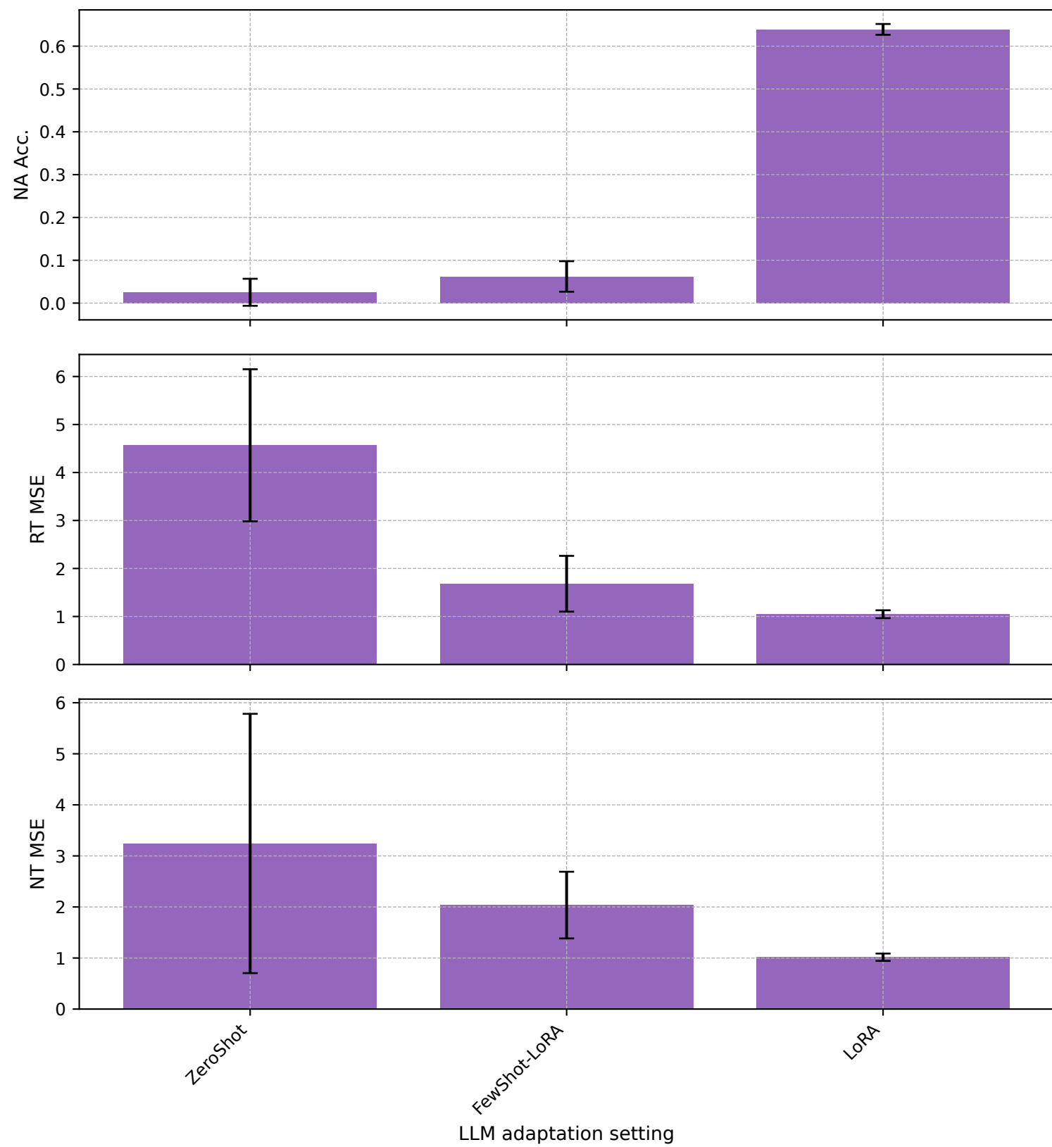
BPI20TravelPermitData - gemma-2-2b
