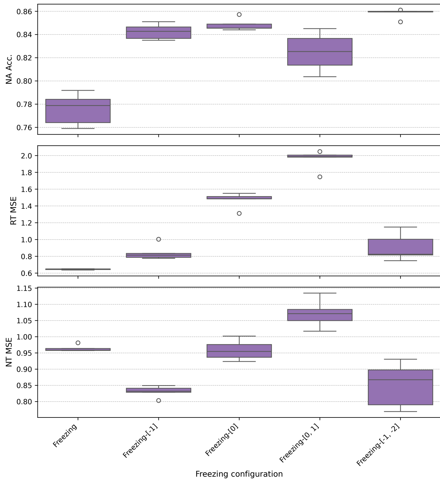
BPI17 - gpt2 (Freezing variants)
