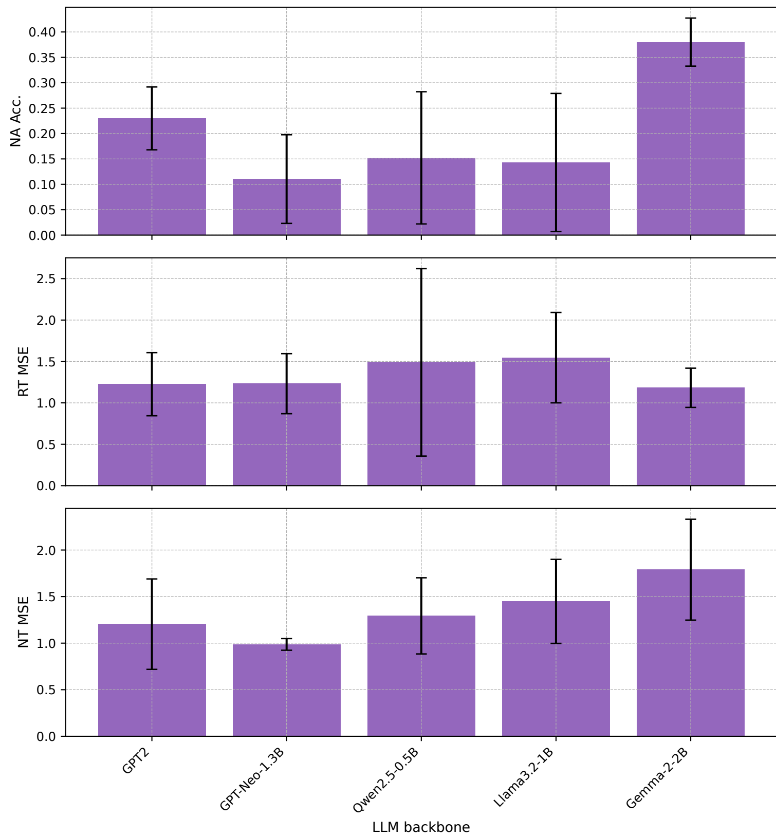
BPI20RequestForPayment - FewShot-LoRA
