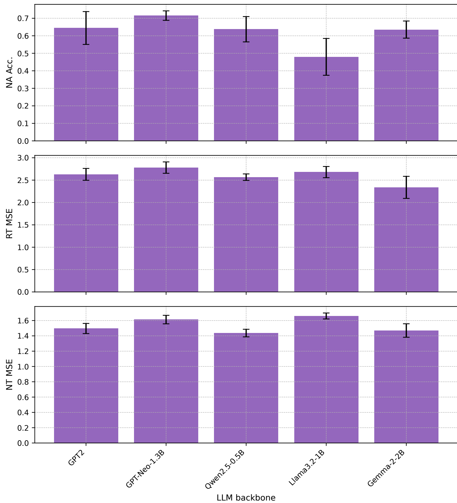
BPI12 - LoRA
