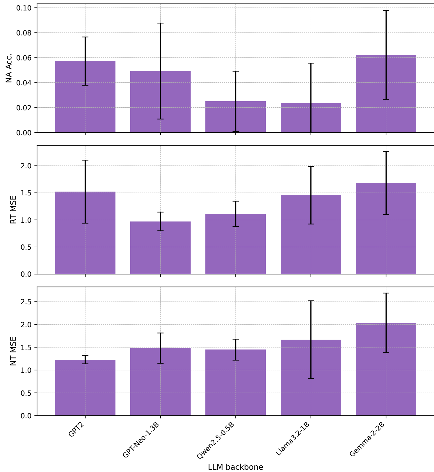
BPI20TravelPermitData - FewShot-LoRA
