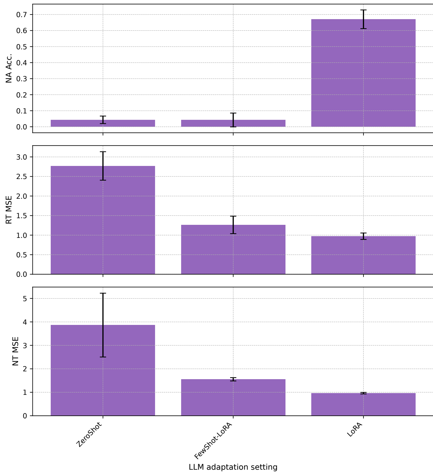
BPI20PrepaidTravelCosts - qwen25-05b
