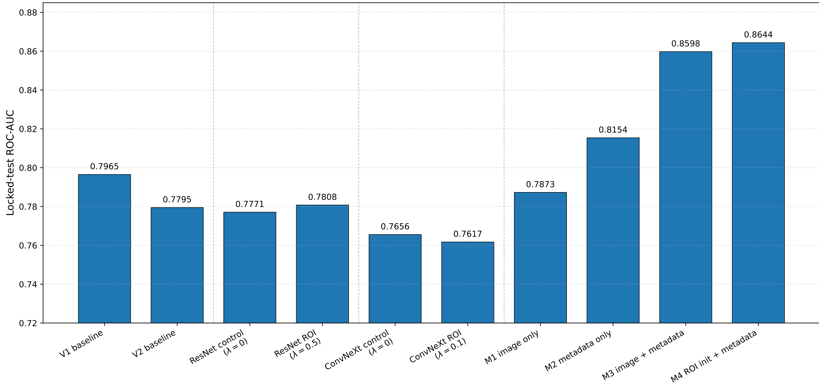
Locked-test ROC-AUC across principal CBIS-DDSM classification configurations
