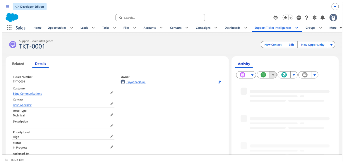
Figure 4. Detail page of ticket TKT-0001: customer, contact, issue type, priority level, status and owner.
