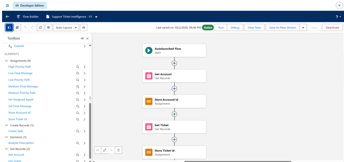
Figure 6. Flow Builder: Autolaunched Flow start, Get Account, Store Account Id, Get Ticket and Store Ticket Id.
