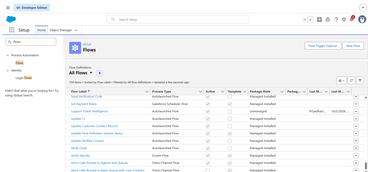
Figure 5. Flows list in Setup showing the Support Ticket Intelligence autolaunched flow (Autolaunched Flow, Active, Unmanaged).
