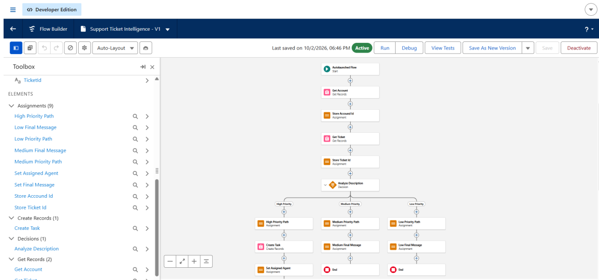
Figure 7. Full flow (version 1, Active) with the High, Medium and Low priority branches, Create Task and Set Assigned Agent on the High path.
