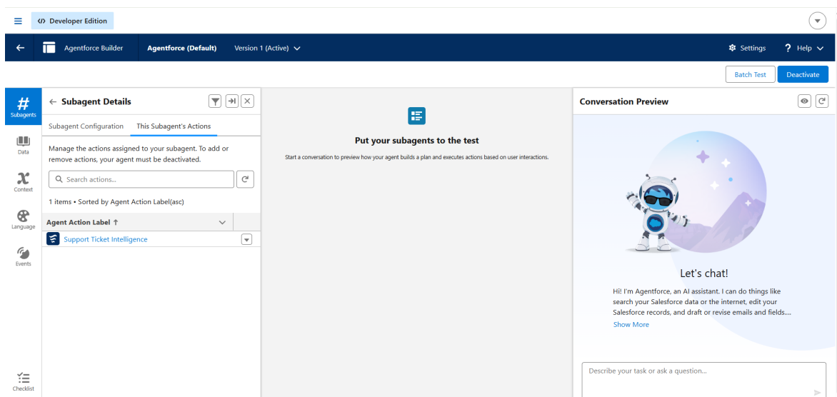
Figure 11. Agentforce Builder for Agentforce (Default), Version 1 (Active), with the subagent actions listing the Support Ticket Intelligence action and the conversation preview.
