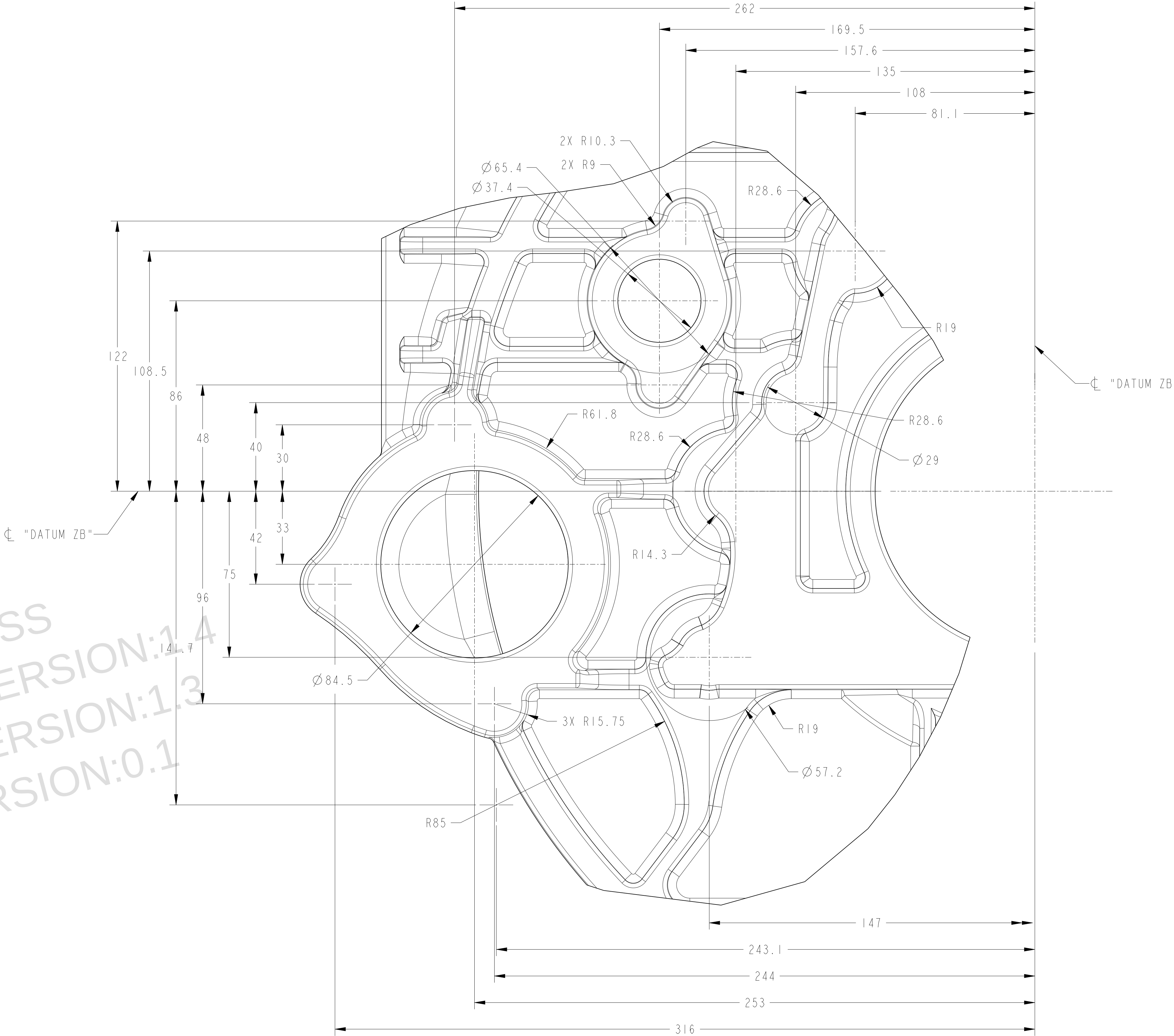
DETAIL K SCALE 1 SEE SHEET 1
