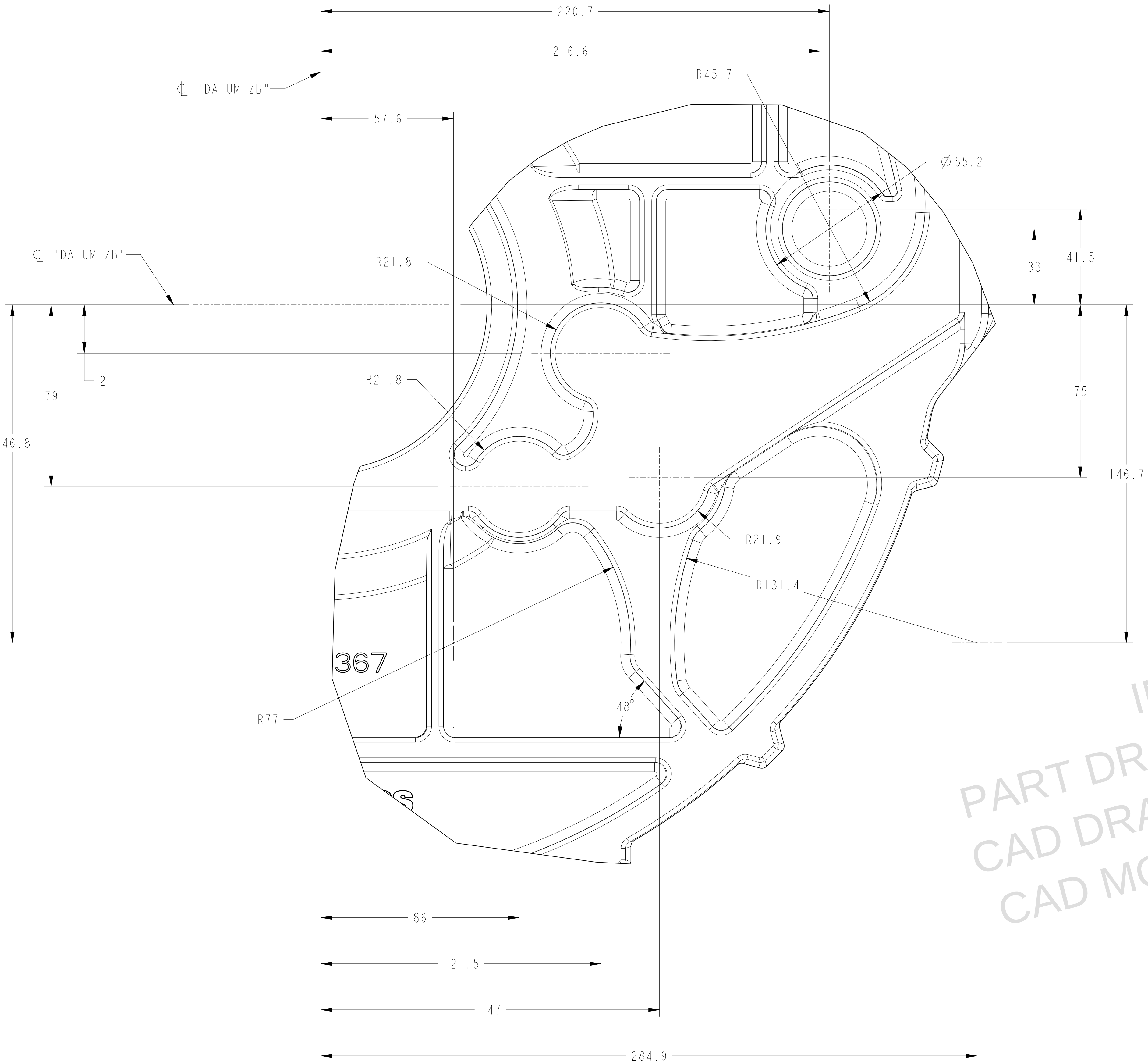
DETAIL L SCALE 1 SEE SHEET 1
