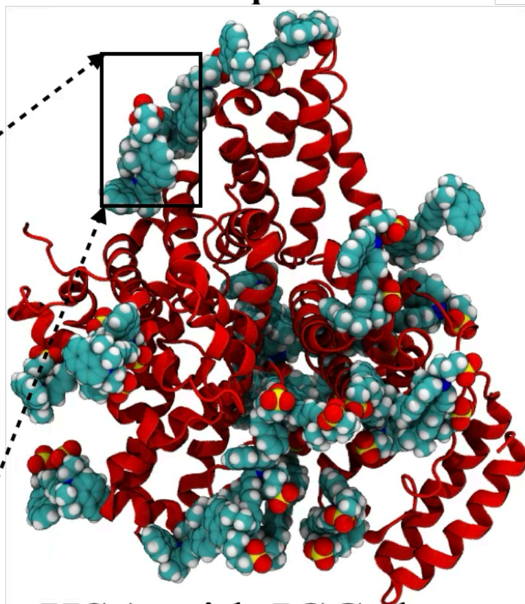
HSA with ICG dye
