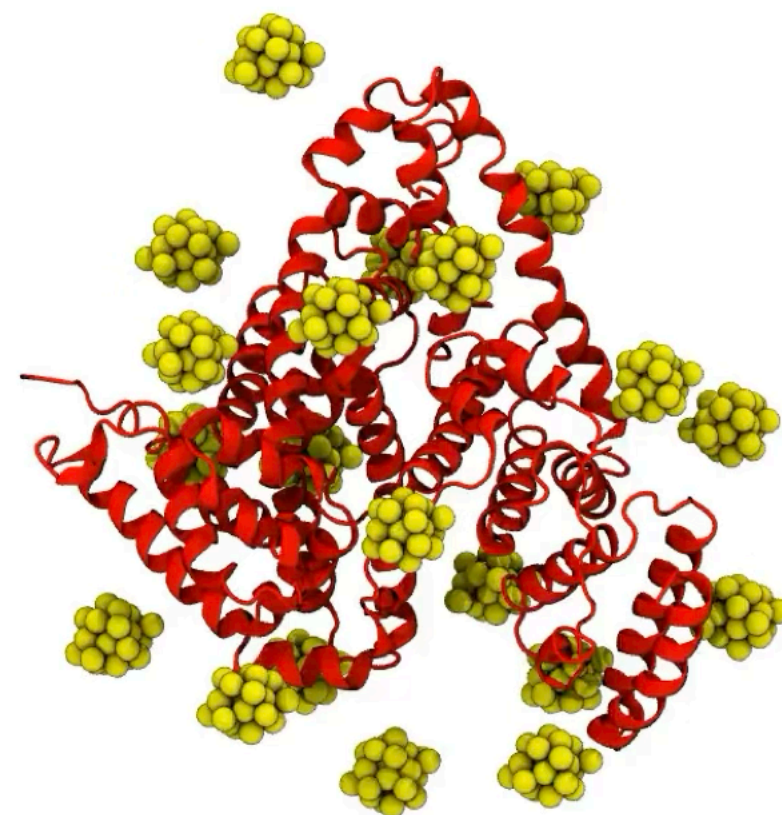
HSA with AuNanocluster
