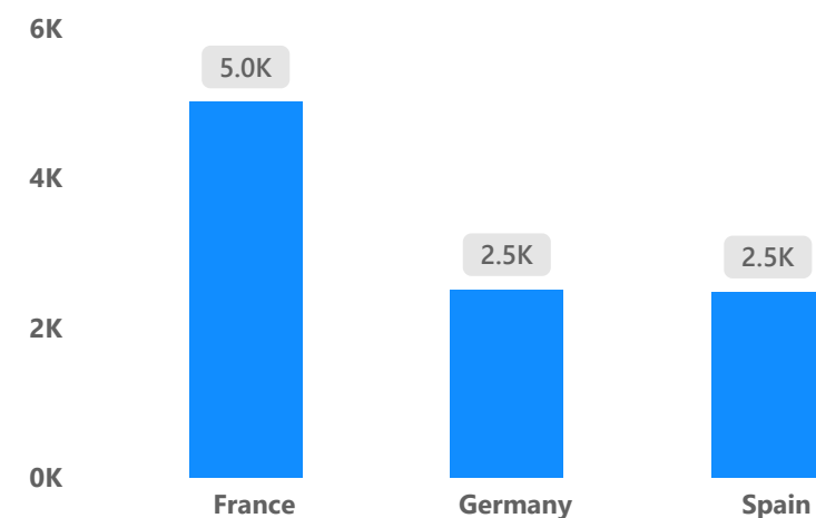
Total Customers by Geography
