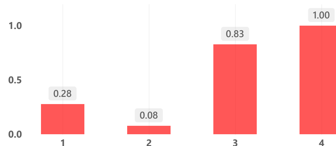
Churn Rate by NumOfProducts
