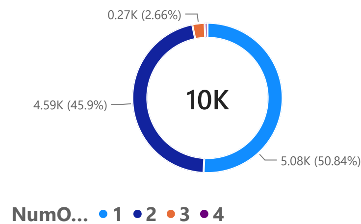
Number of Product Distribution
