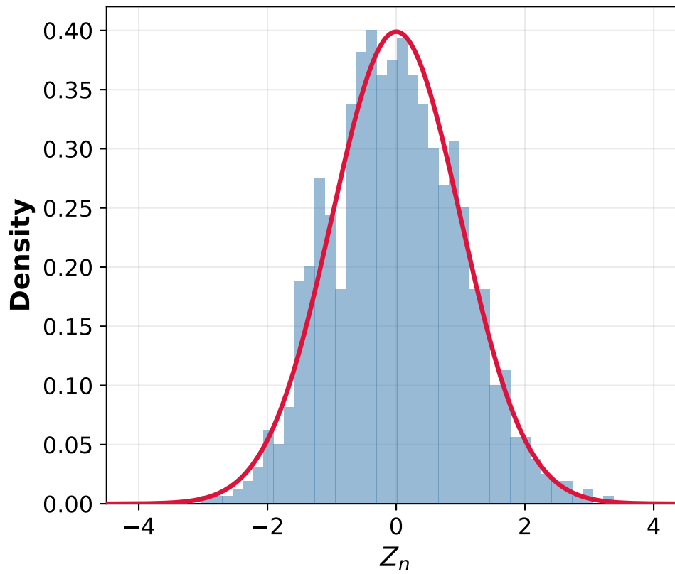
D7 Logarithmic, n = 1000
