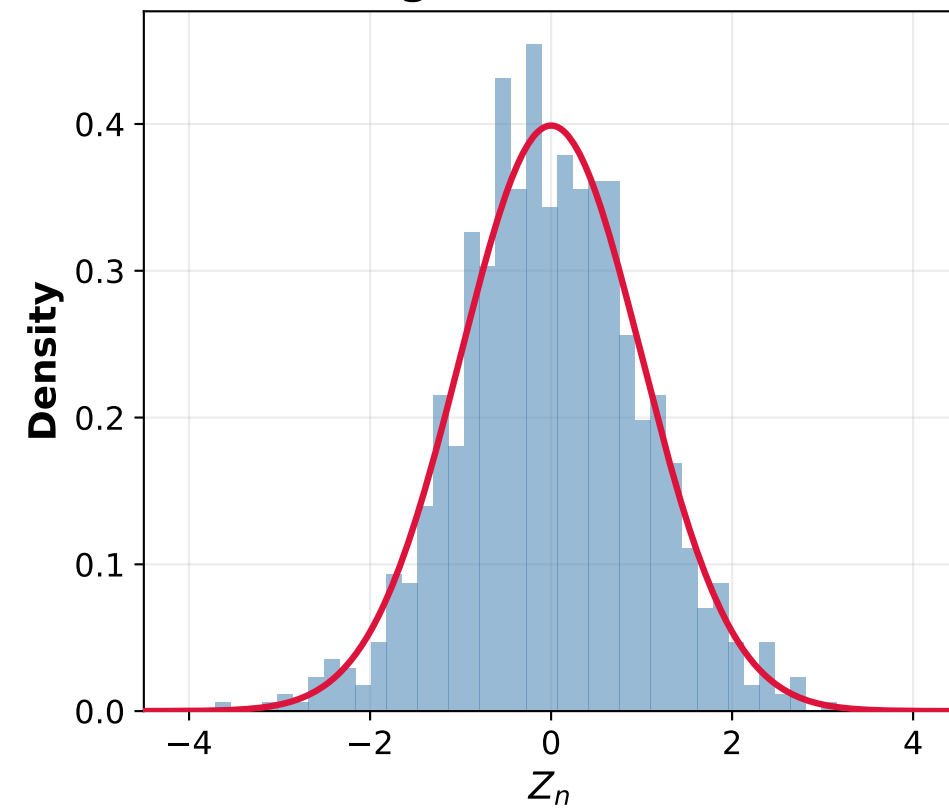
D7 Logarithmic, n = 500
