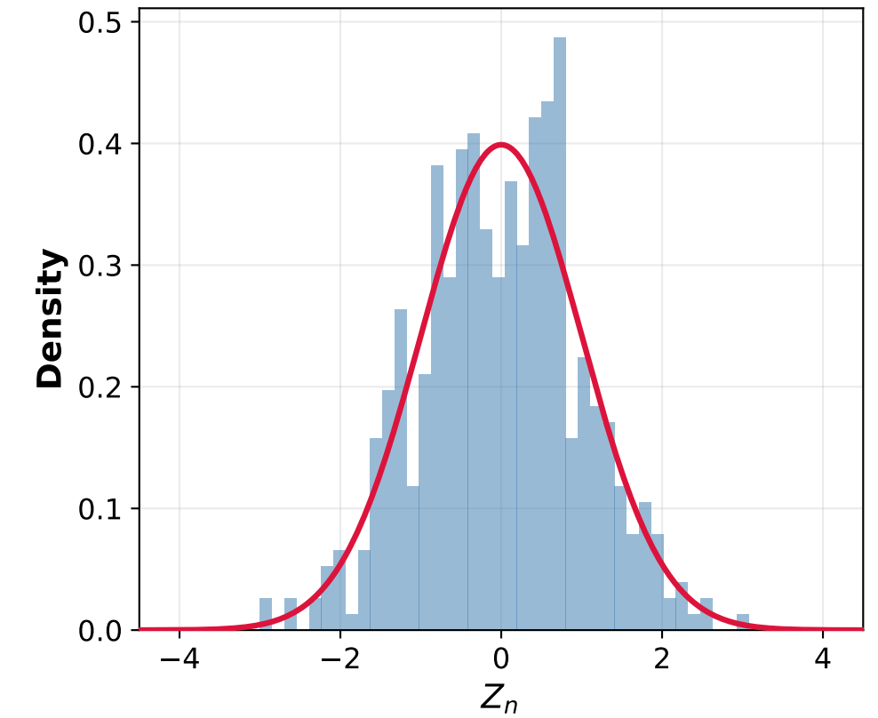
D7 Logarithmic, n = 5000
