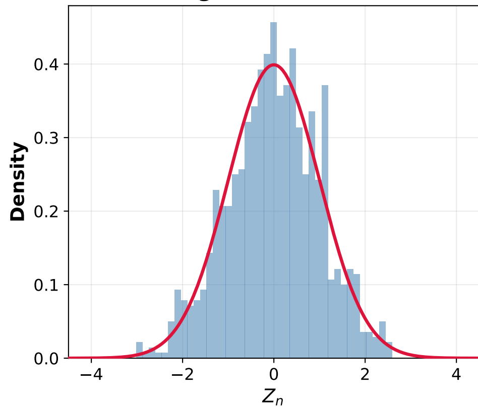
D7 Logarithmic, n = 100
