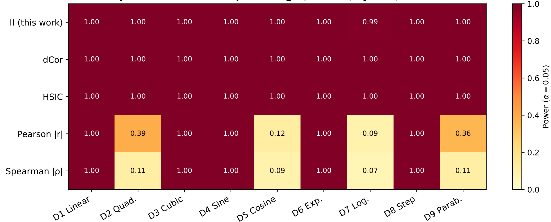
Exp 6 — Power heatmap (Setting A, n = 500 , \sigma_\varepsilon = 0.5 , \alpha = 0.05 )
