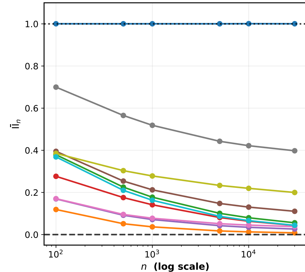
Convergence \sigma_\varepsilon = 0.1
