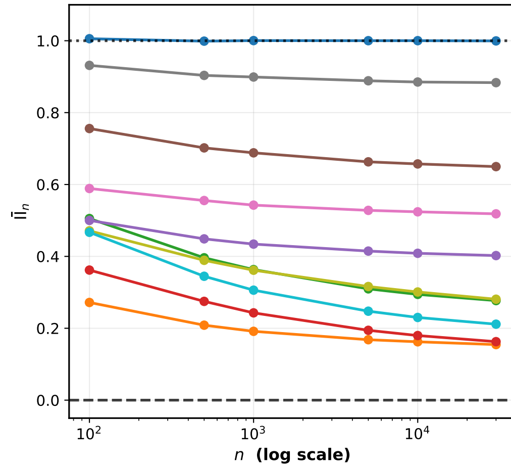
Convergence \sigma_\varepsilon = 0.5
