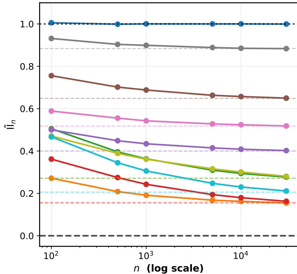
Convergence \sigma_\varepsilon = 0.5
