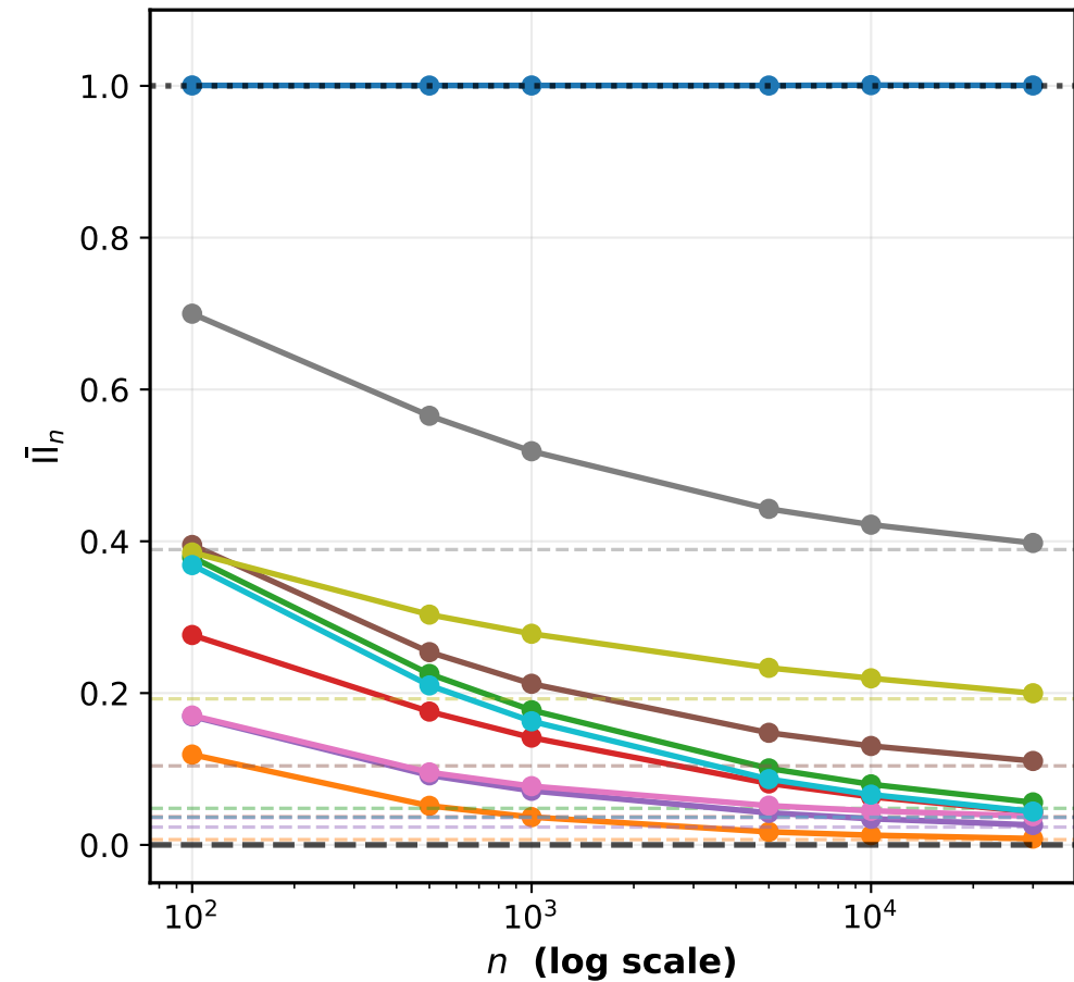
Convergence \sigma_\varepsilon = 0.1
