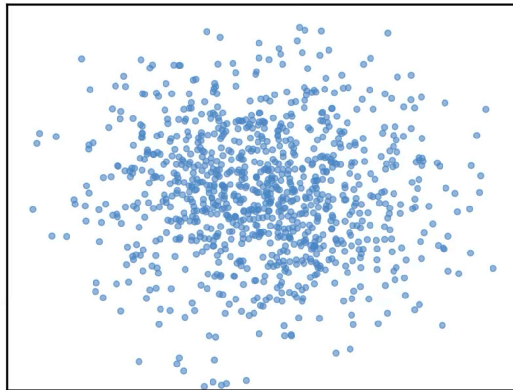
noise
