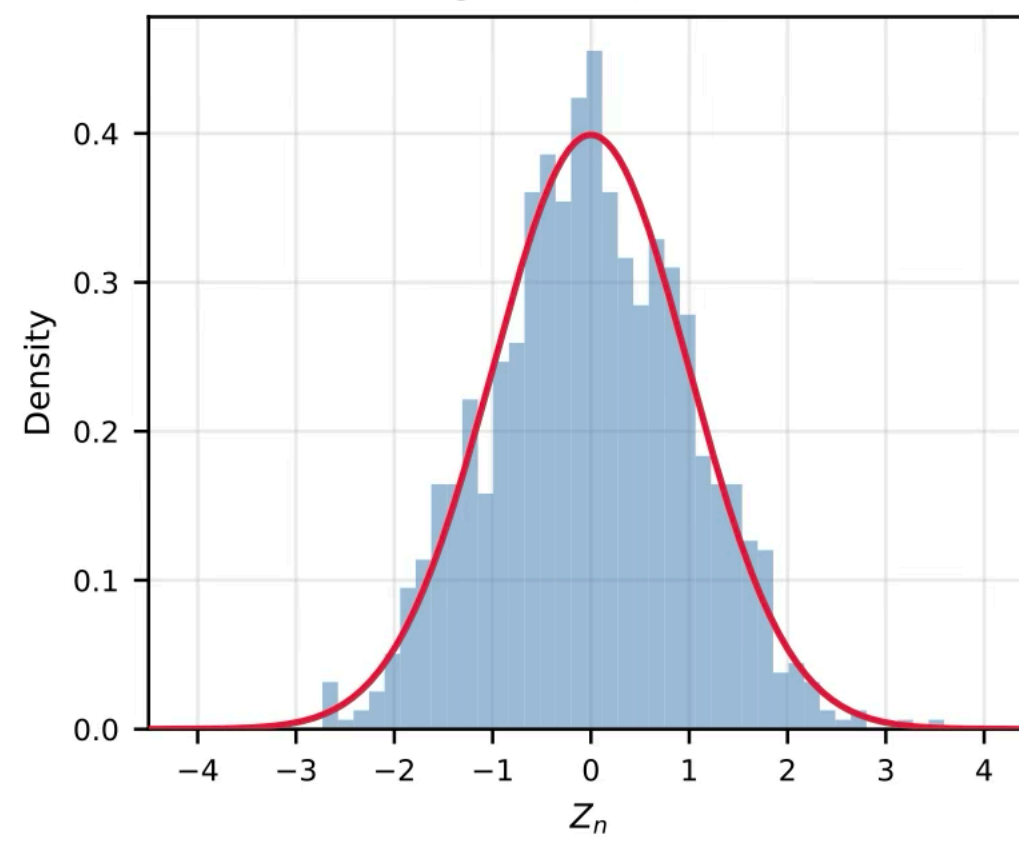
D7 Logarithmic, n = 1000
