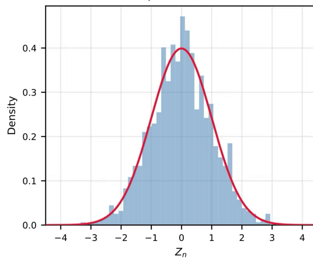
D0 Independent, n = 1000
