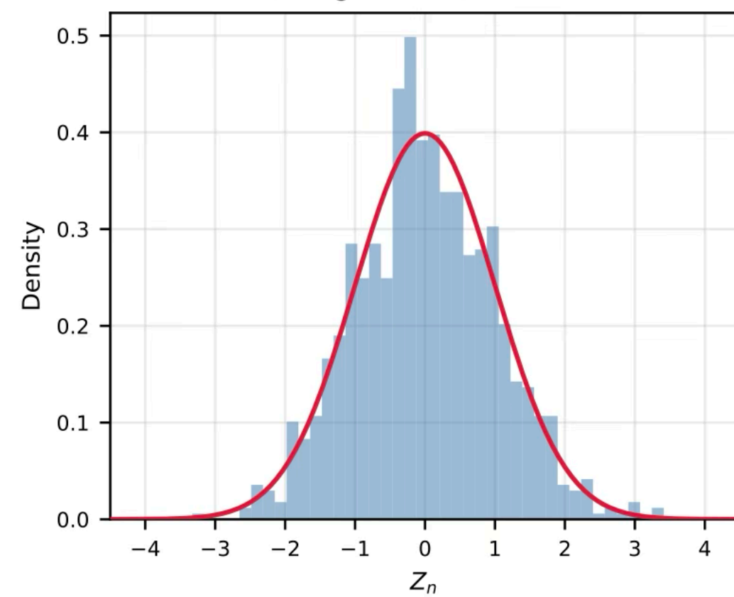
D7 Logarithmic, n = 100
