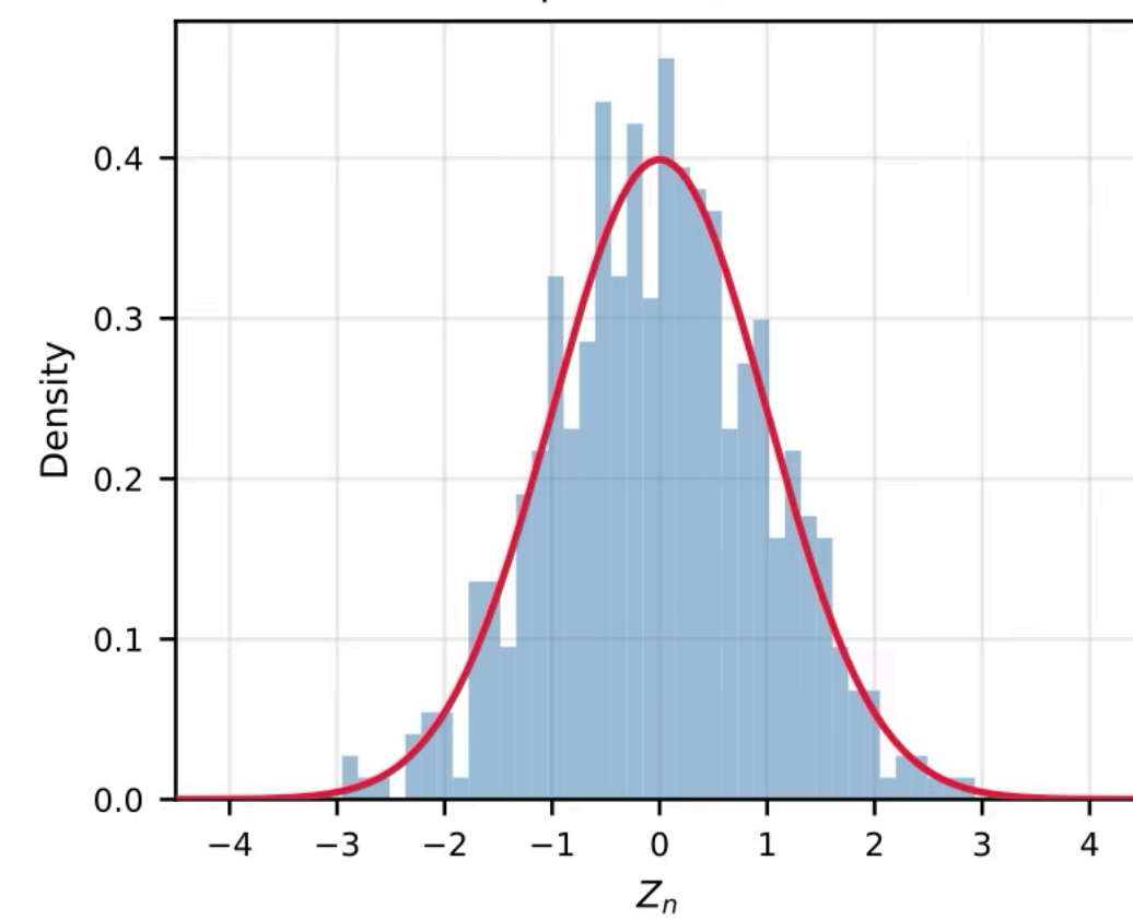
D0 Independent, n = 5000
