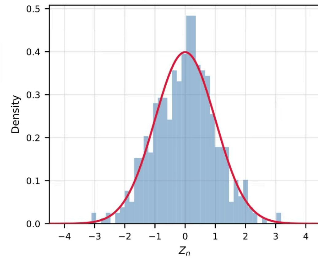
D7 Logarithmic, n = 5000
