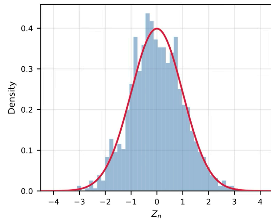
D0 Independent, n = 100
