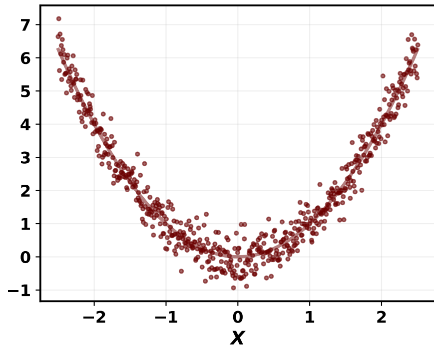
Quadratic ( Y = X^2 )
