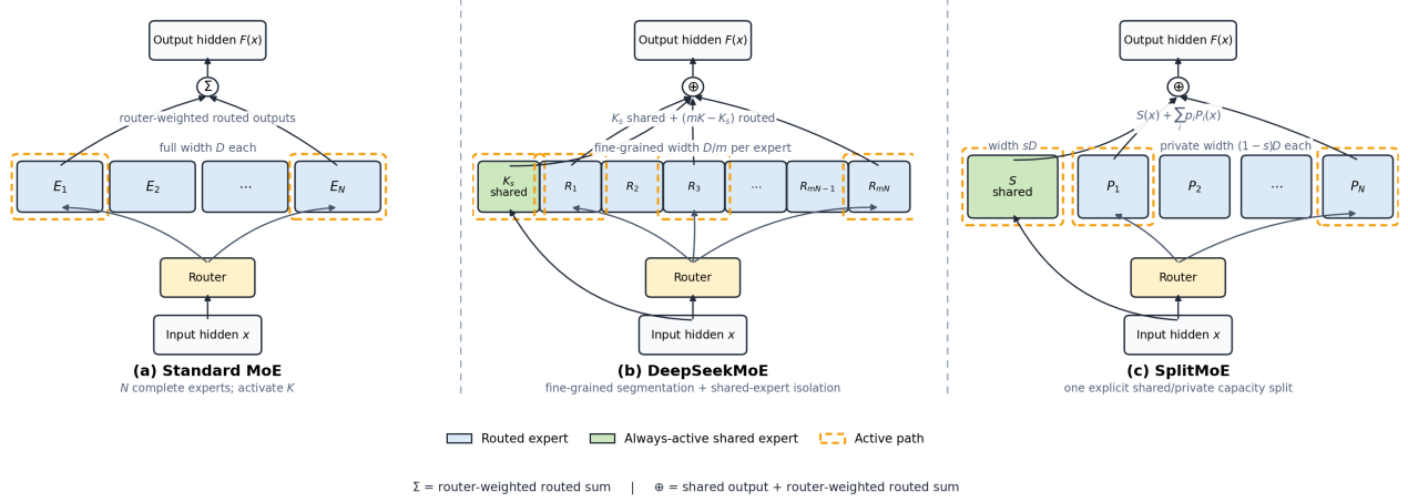
Figure 1: Expert-bank view of Standard MoE, DeepSeekMoE, and SplitMoE. DeepSeekMoE combines fine-grained expert segmentation with isolated always-active shared experts. SplitMoE does not multiply the expert bank into fine-grained segments; it explicitly divides a target active width into one width- sD shared FFN and width- (1-s)D private FFNs. Orange dashed outlines mark active paths, and \oplus adds the shared output to the router-weighted routed outputs.
