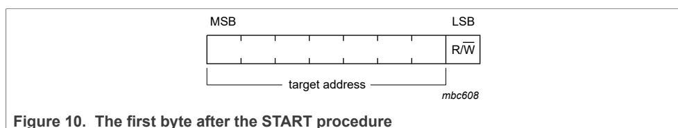
Figure 10. The first byte after the START procedure
