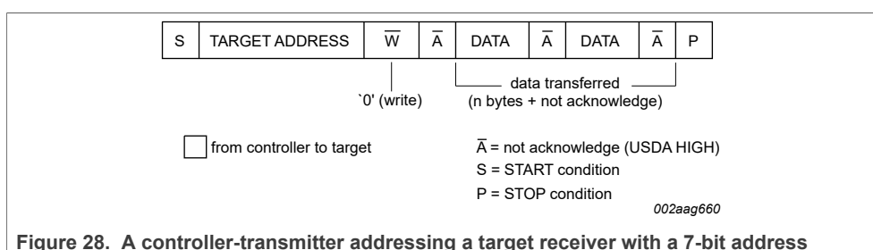
Figure 28. A controller-transmitter addressing a target receiver with a 7-bit address
