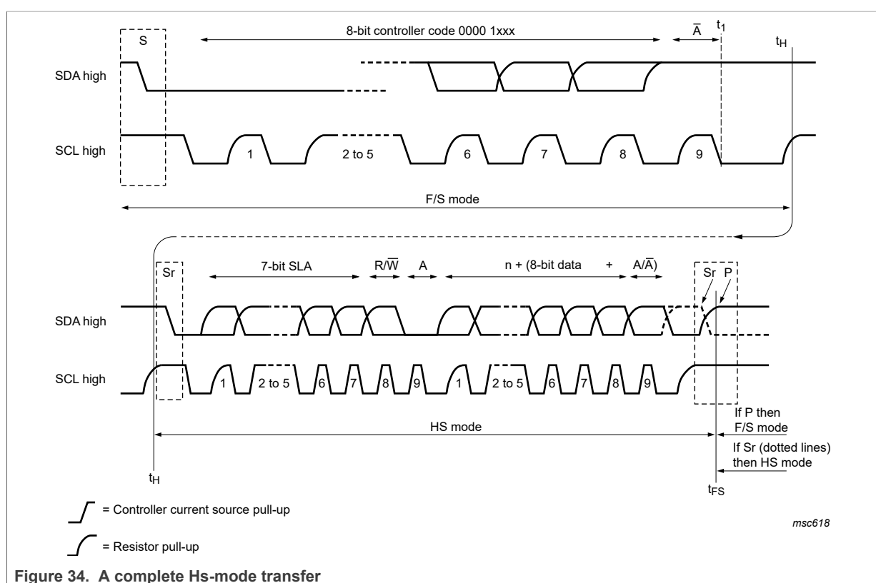
Figure 34. A complete Hs-mode transfer
