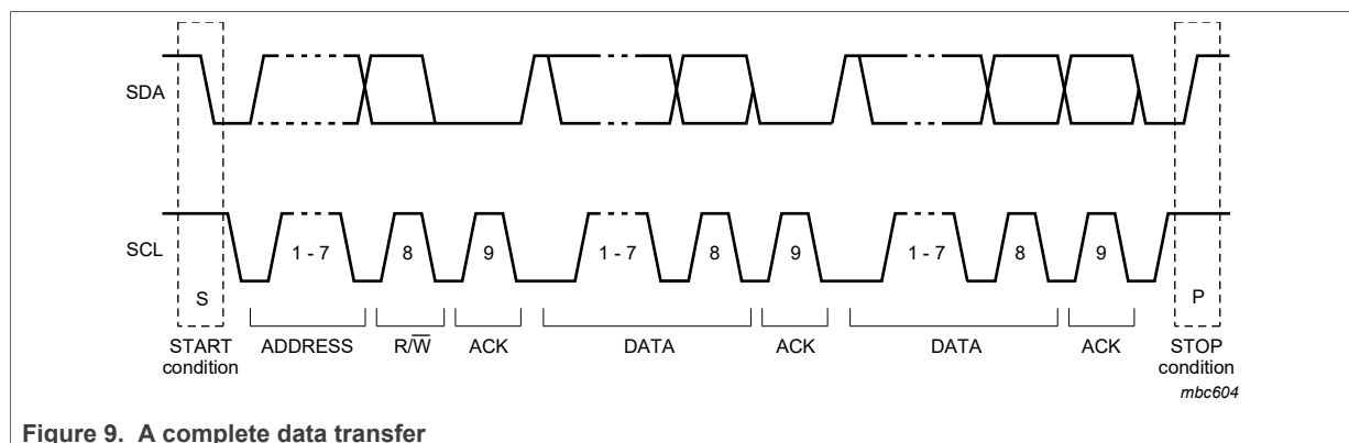
Figure 9. A complete data transfer
