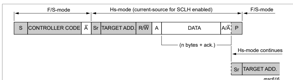
Figure 33. Data transfer format in Hs-mode
