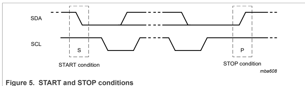
Figure 5. START and STOP conditions
