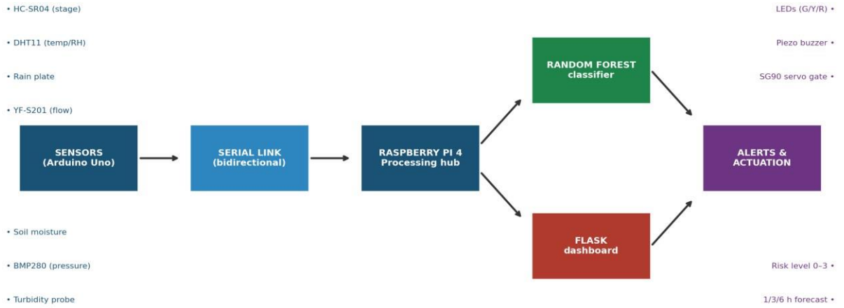
Figure 1. System architecture of the prototype. Sensor data flow left to right from the Arduino sensing tier through the Raspberry Pi processing hub to the machine-learning model, dashboard, and physical alert/actuation outputs. The risk level computed on the Pi is returned to the Arduino over the bidirectional serial link.
