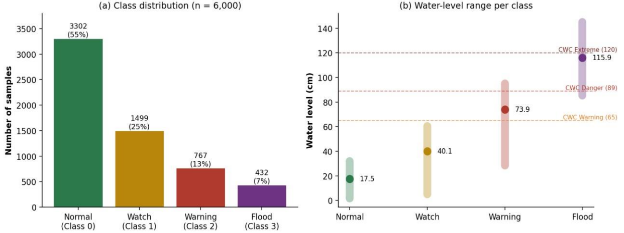
Figure 2. Training a corpus summary. (a) Class distribution over the 6,000 simulated records. (b) Minimum, mean (point), and maximum water level per class, with prototype-scale CWC thresholds for the Teesta at Domohani overlaid.
