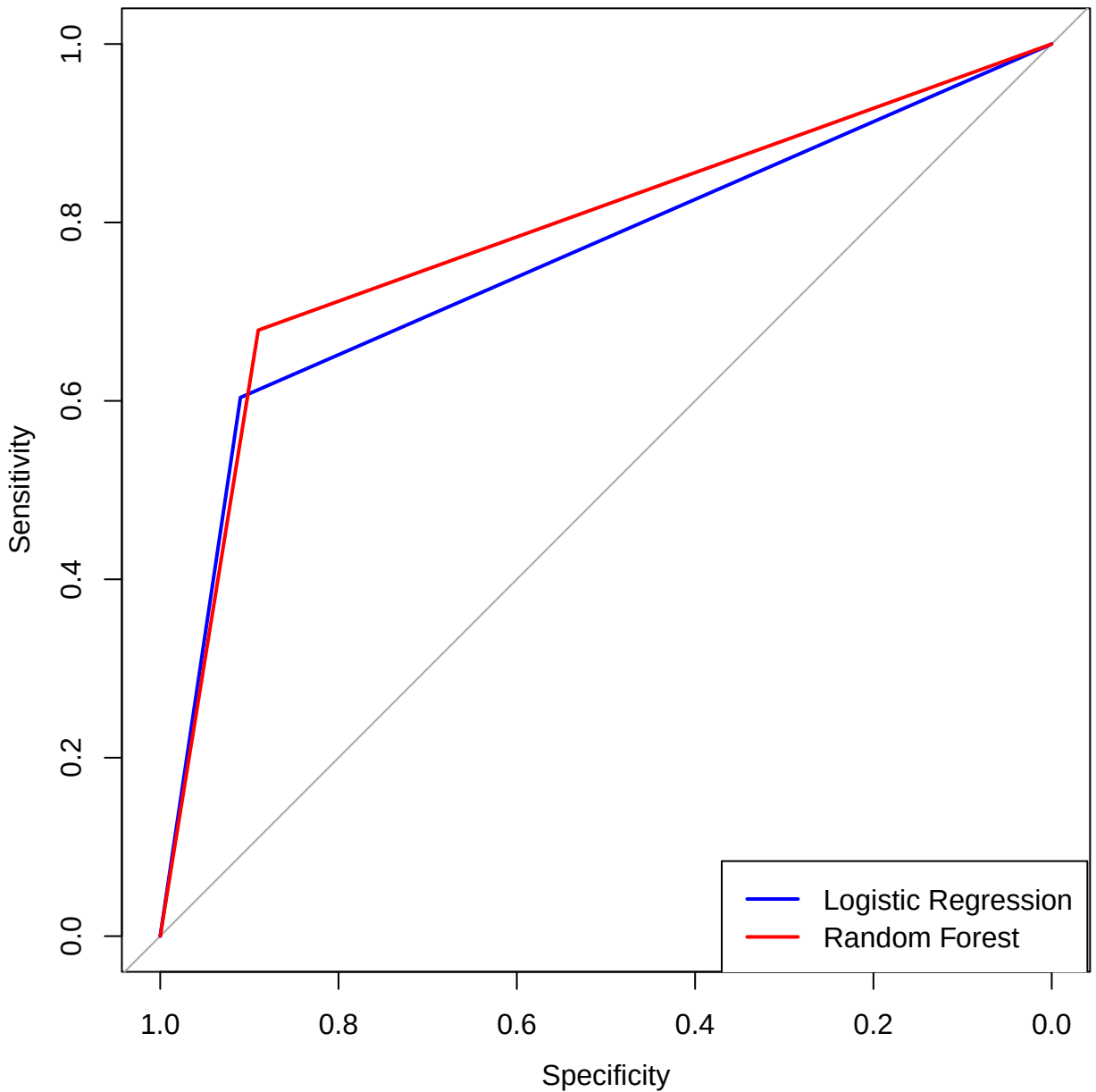
ROC Curves for Models
