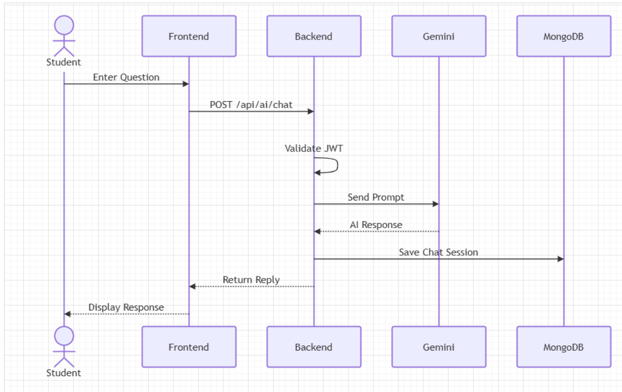
Figure: AI Academic Chatbot
