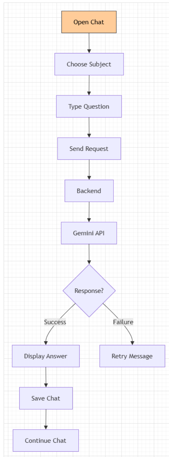
Figure: Chatbot Flow
