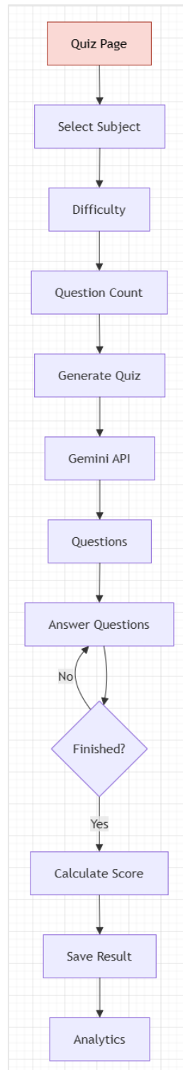
Figure: Quiz Generator Flow
