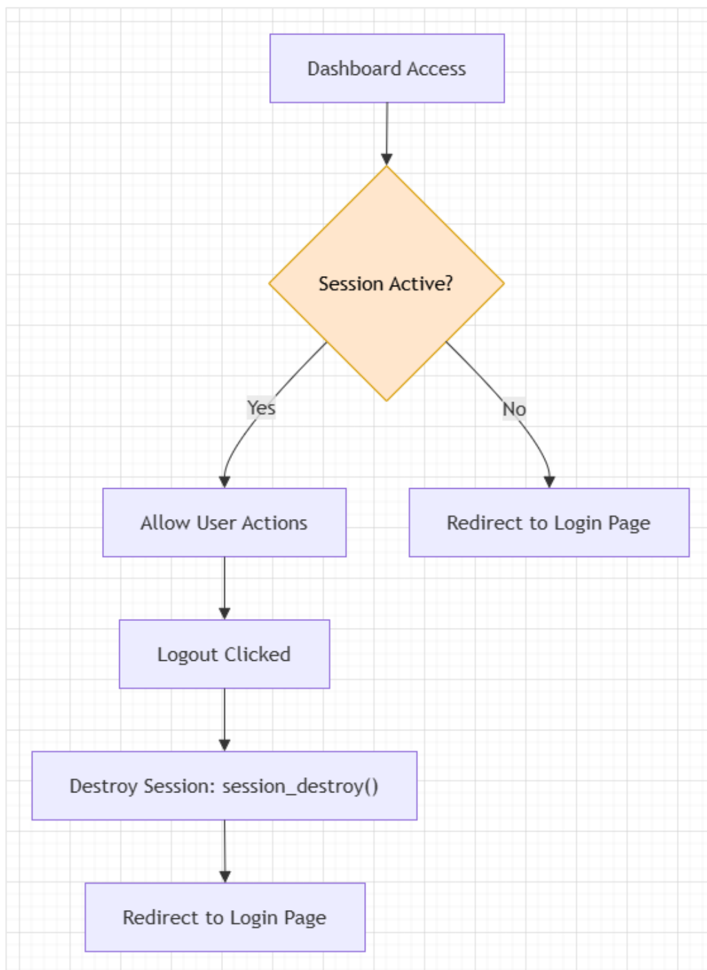
Figure: Session Management
