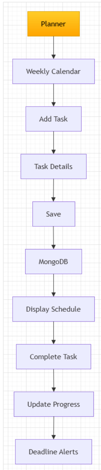
Figure: Study Planner Flow
