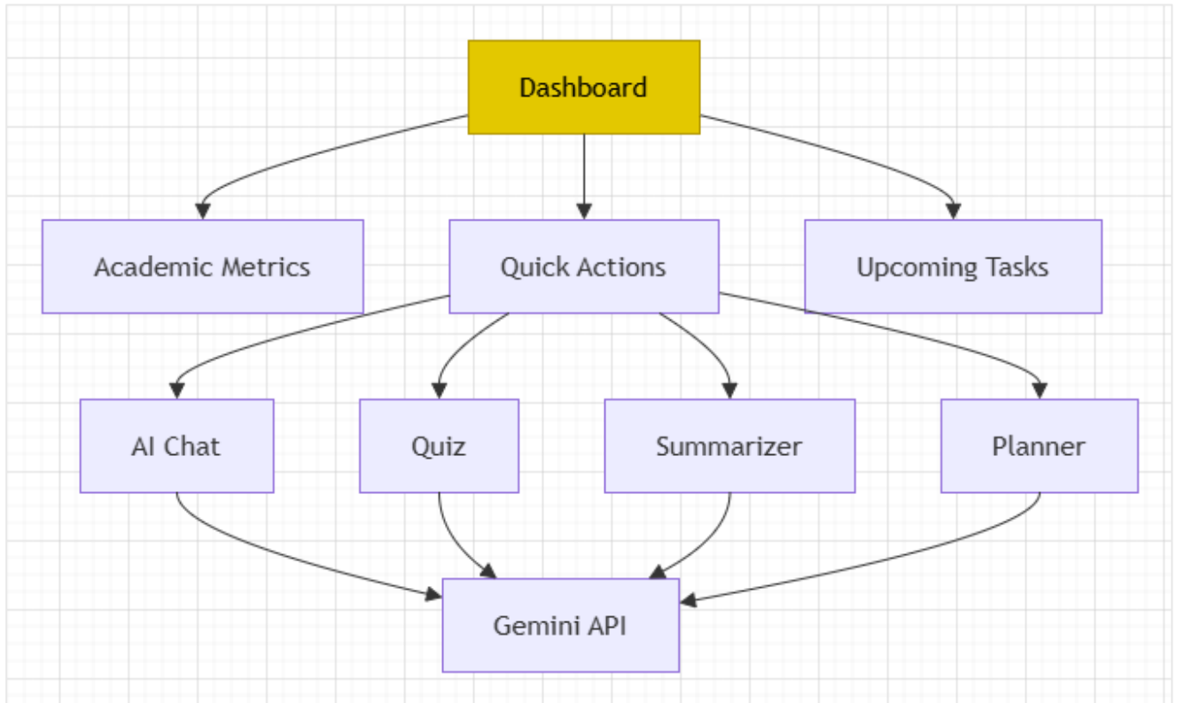
Figure: Dashboard Flow
