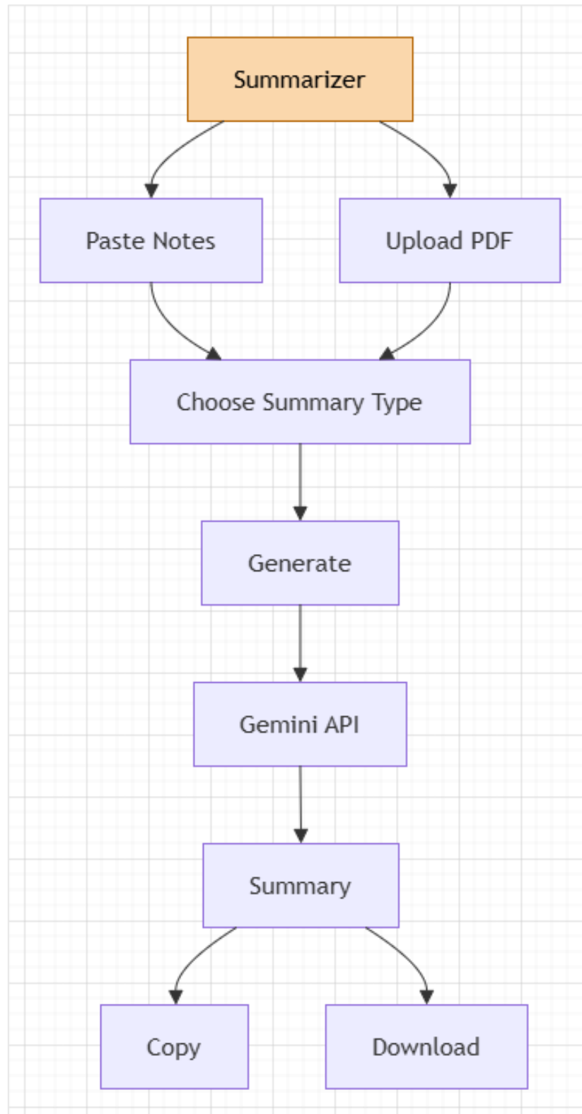
Figure: Note Summarizer Flow
