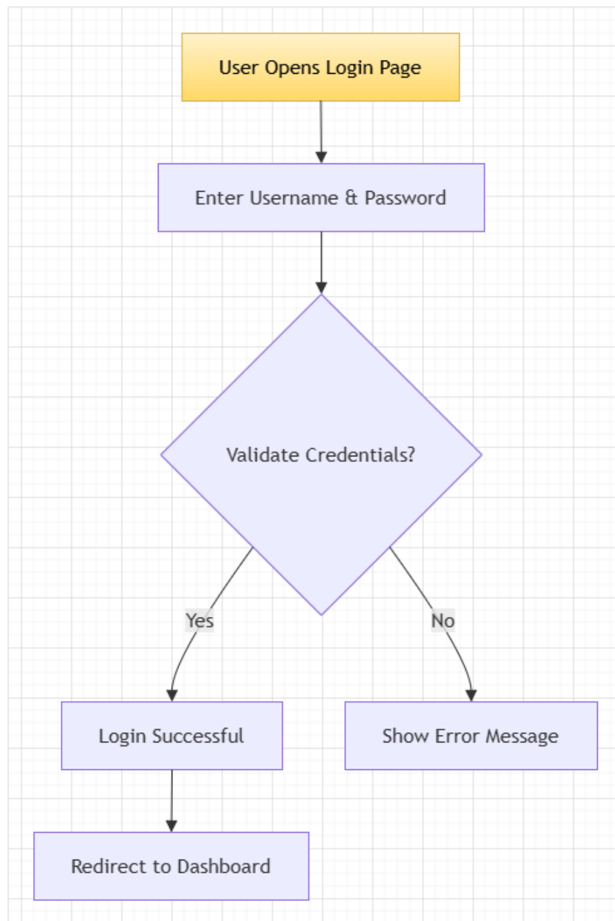
Figure: Login Flow
