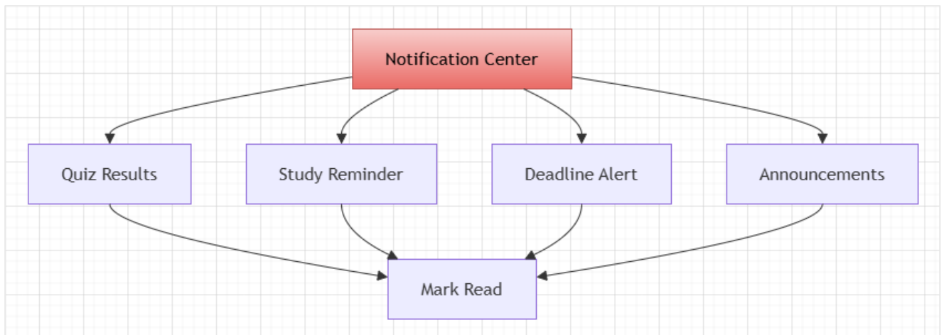
Figure: Notification Flow
