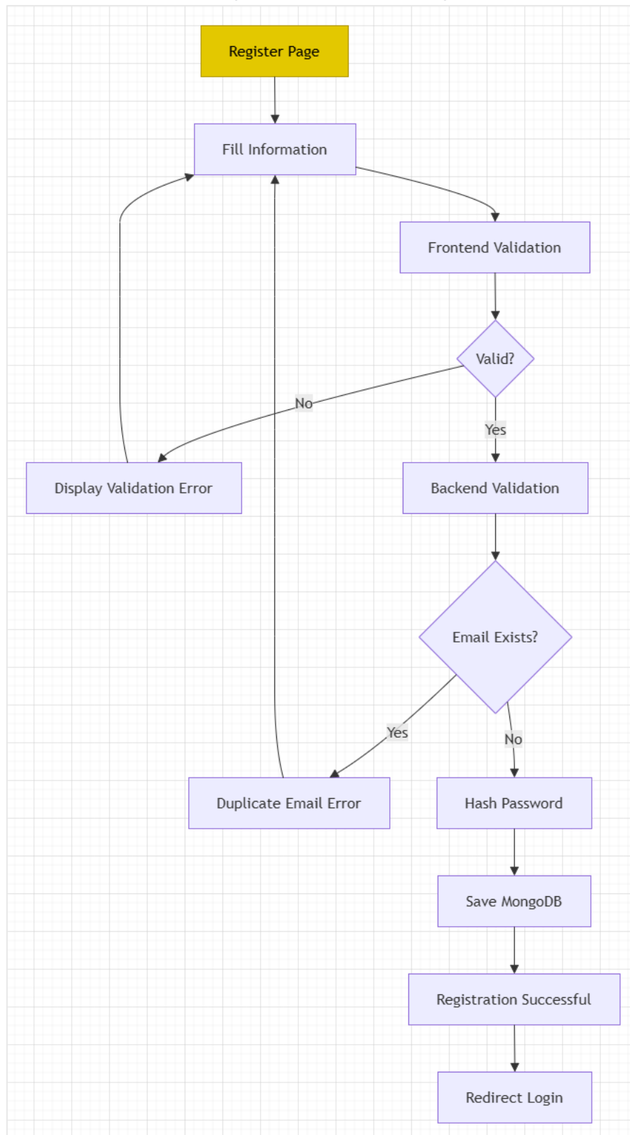
Figure: Registration Flow
