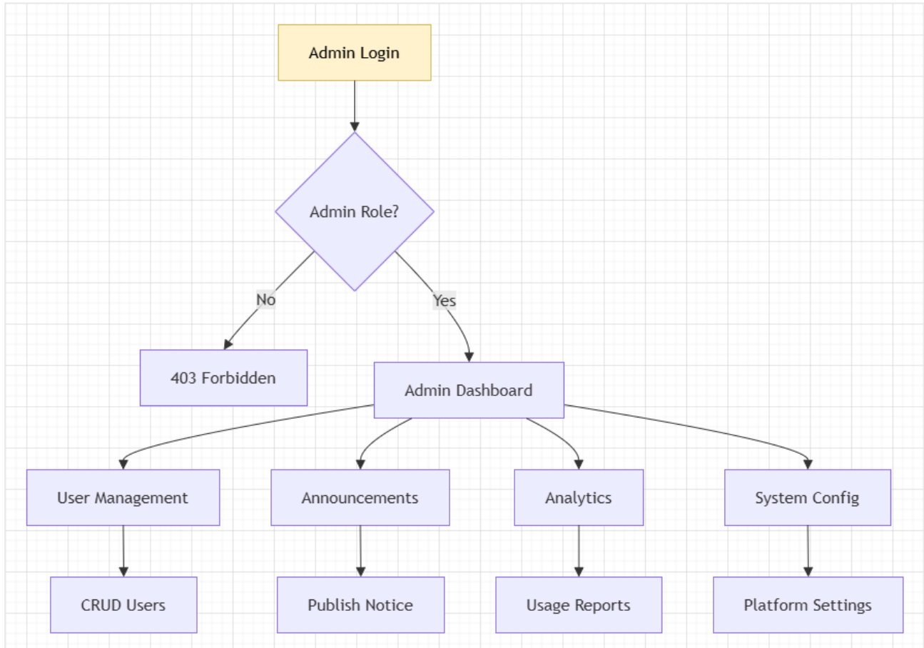
Figure: Admin User Flow
