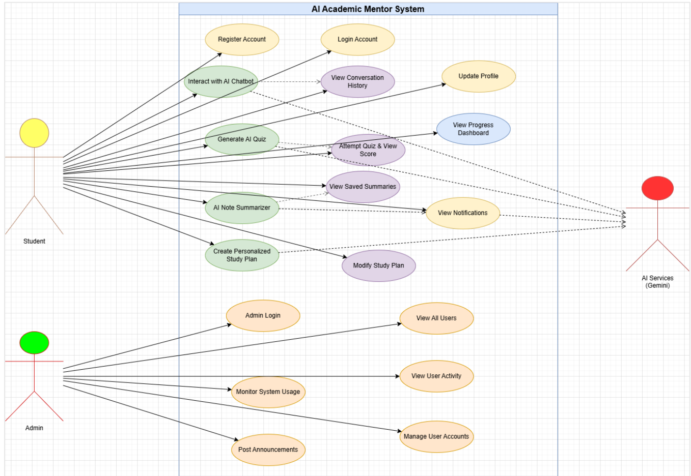
Figure: Use Case Diagram — AI Academic Mentor System
