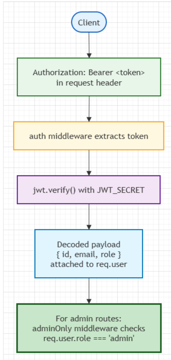
Figure : Protected Route Access Flow
