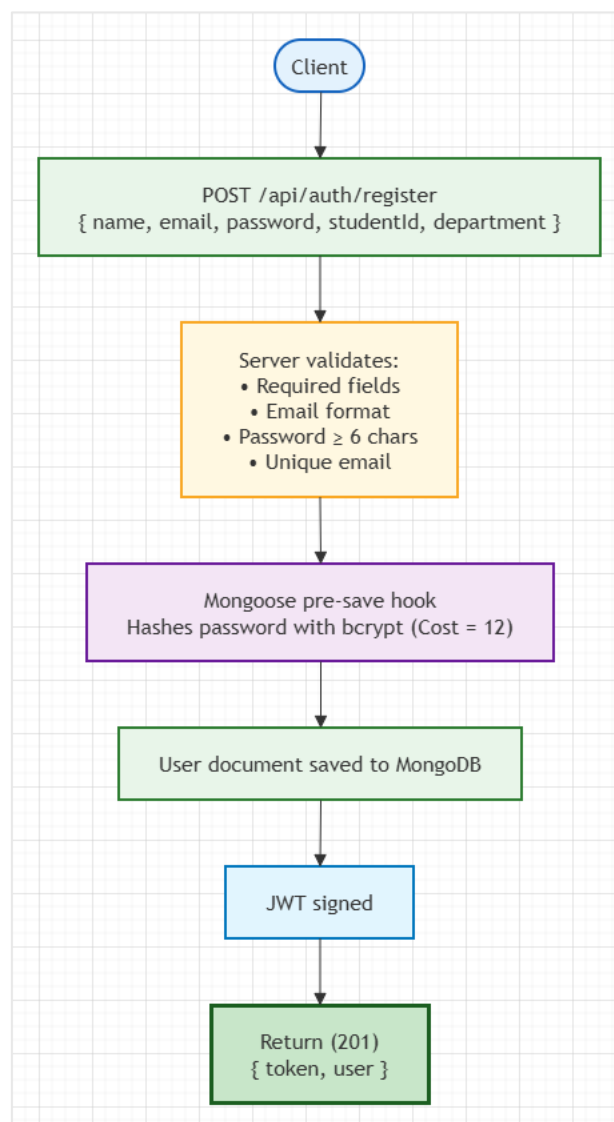
Figure : Registration Flow
