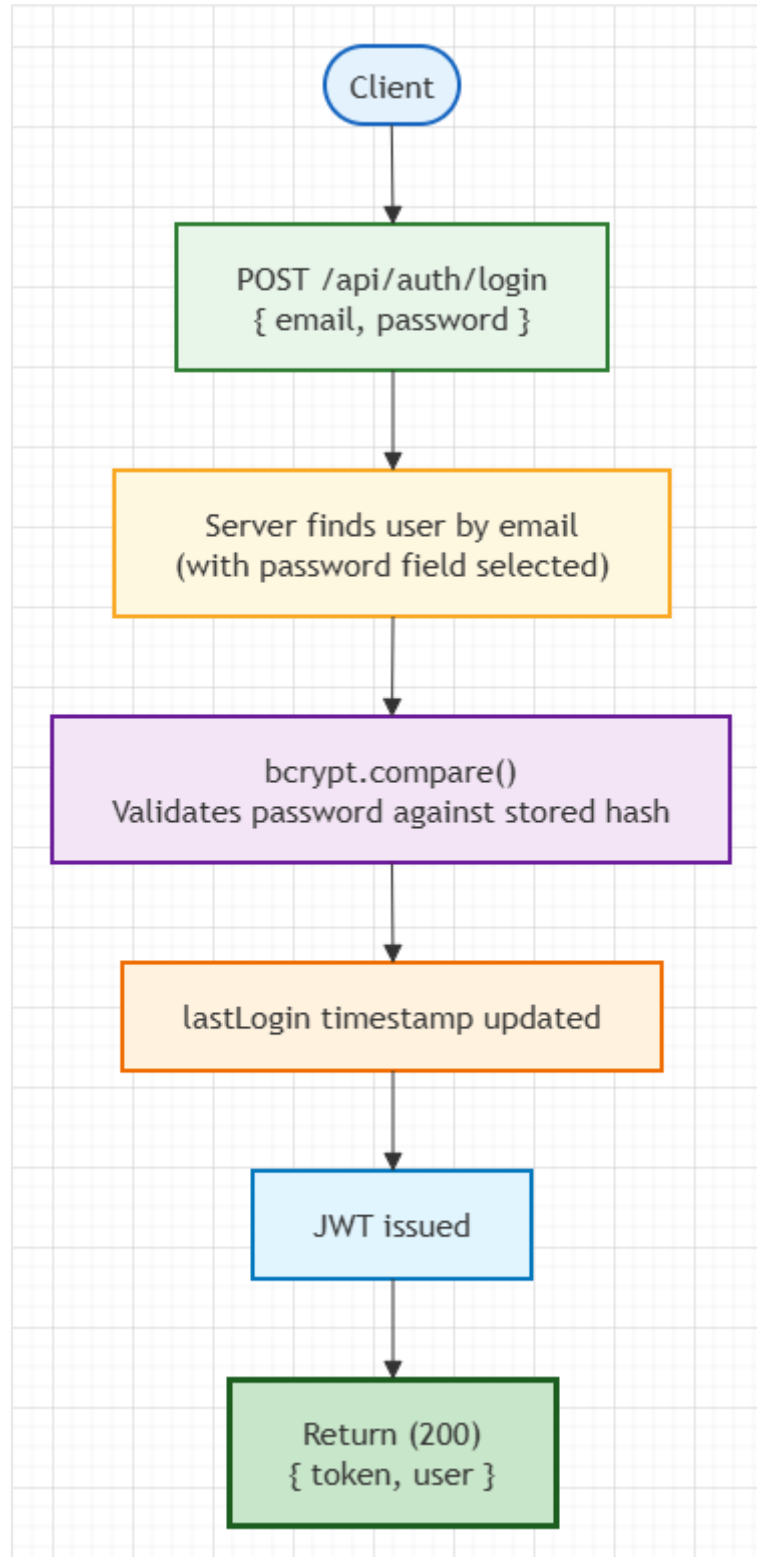
Figure : Login Flow
