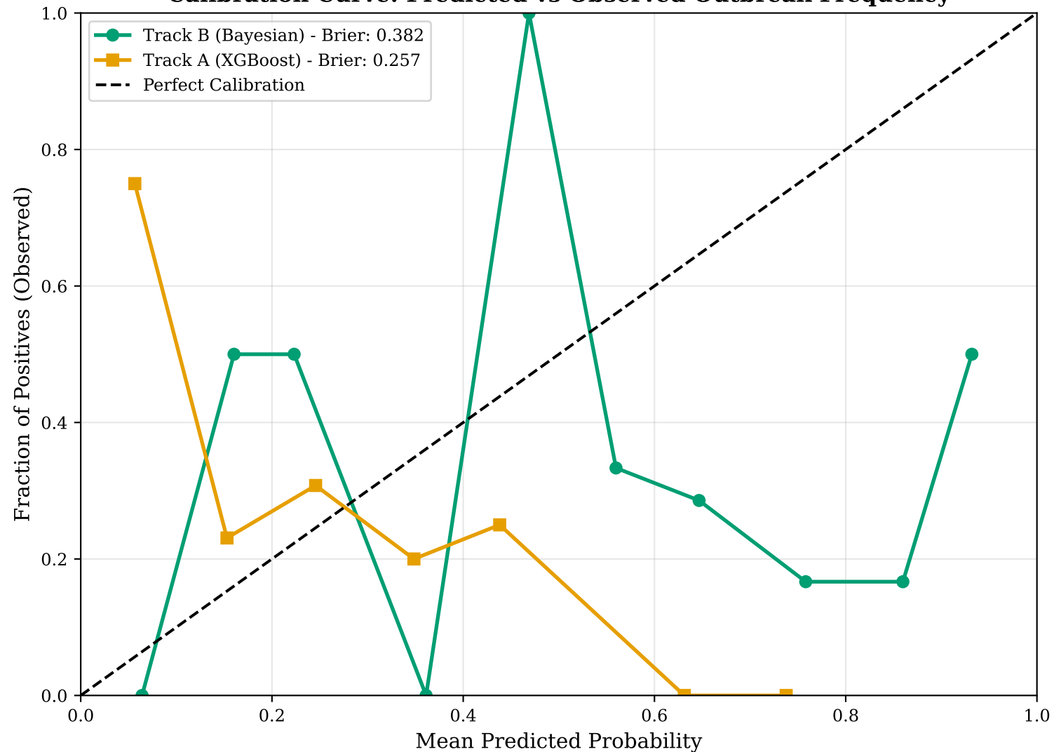
Calibration Curve: Predicted vs Observed Outbreak Frequency
