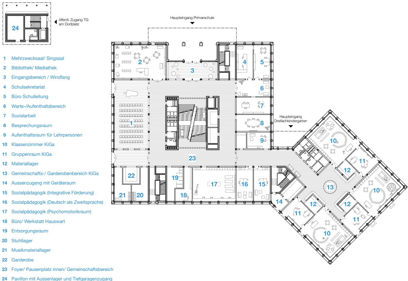
Abb. 6: Erdgeschoss
